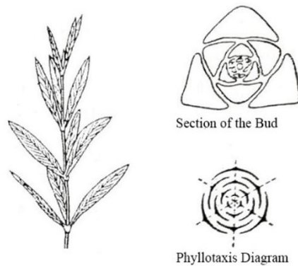
Fig. 5: Leaf arrangement in a ternary cycle (Ghahraman, 2012)
