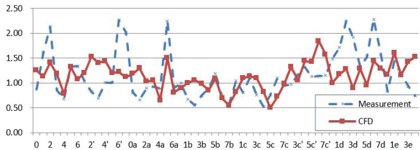
Fig.8: Wind speed comparison between measurement and numerical simulation of each point
