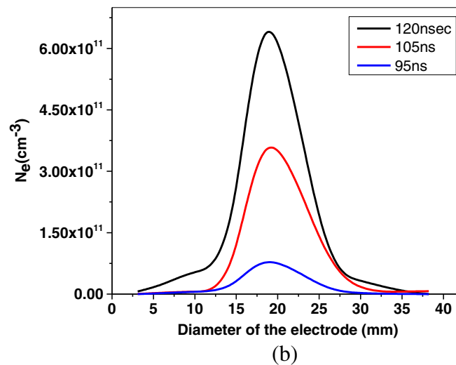
Figure 6 Parallel plate DBD simulations. (a) After discharge effects in the similar geometry of the experimental set-up. (b) Gaussian electron plasma density profile after discharge at different time steps.
