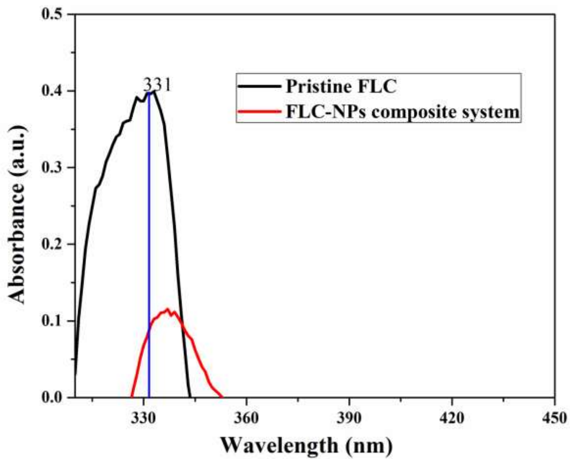
Fig. 3 Variation of absorbance with wavelength for pristine FLC and FLC-NPs composite system.
