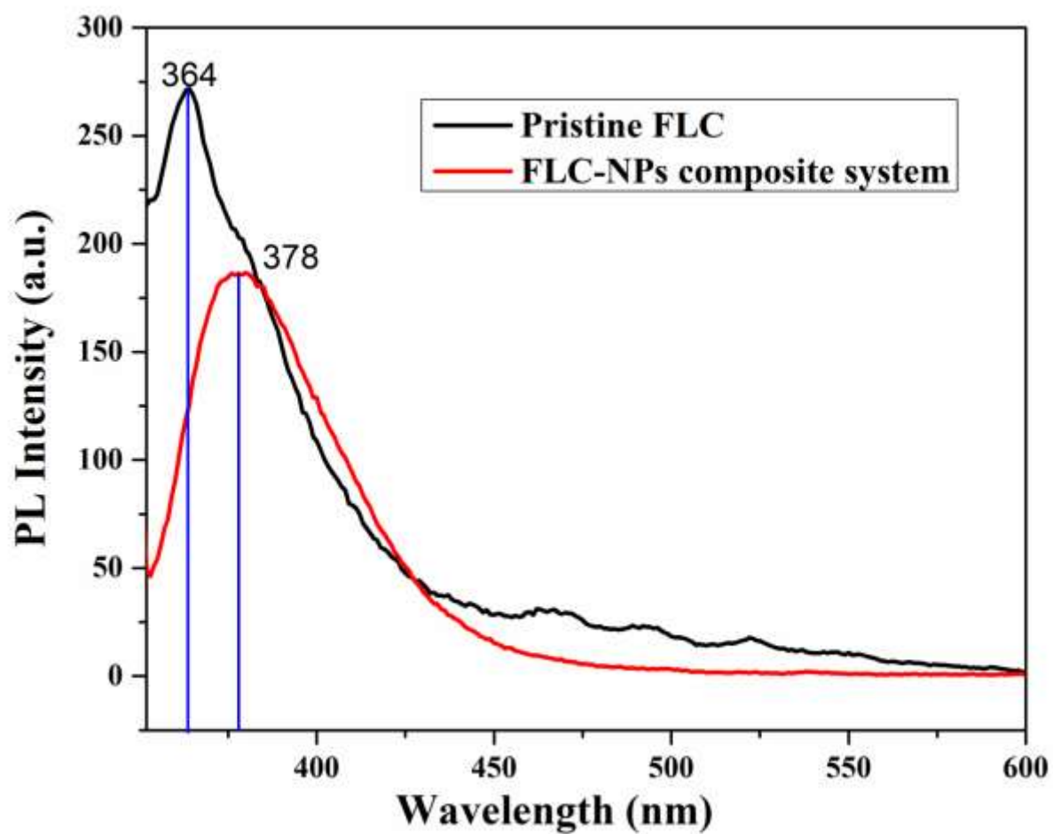
Fig. 4 Variation of PL intensity with wavelength for pristine FLC and FLC-NPs composite system.
