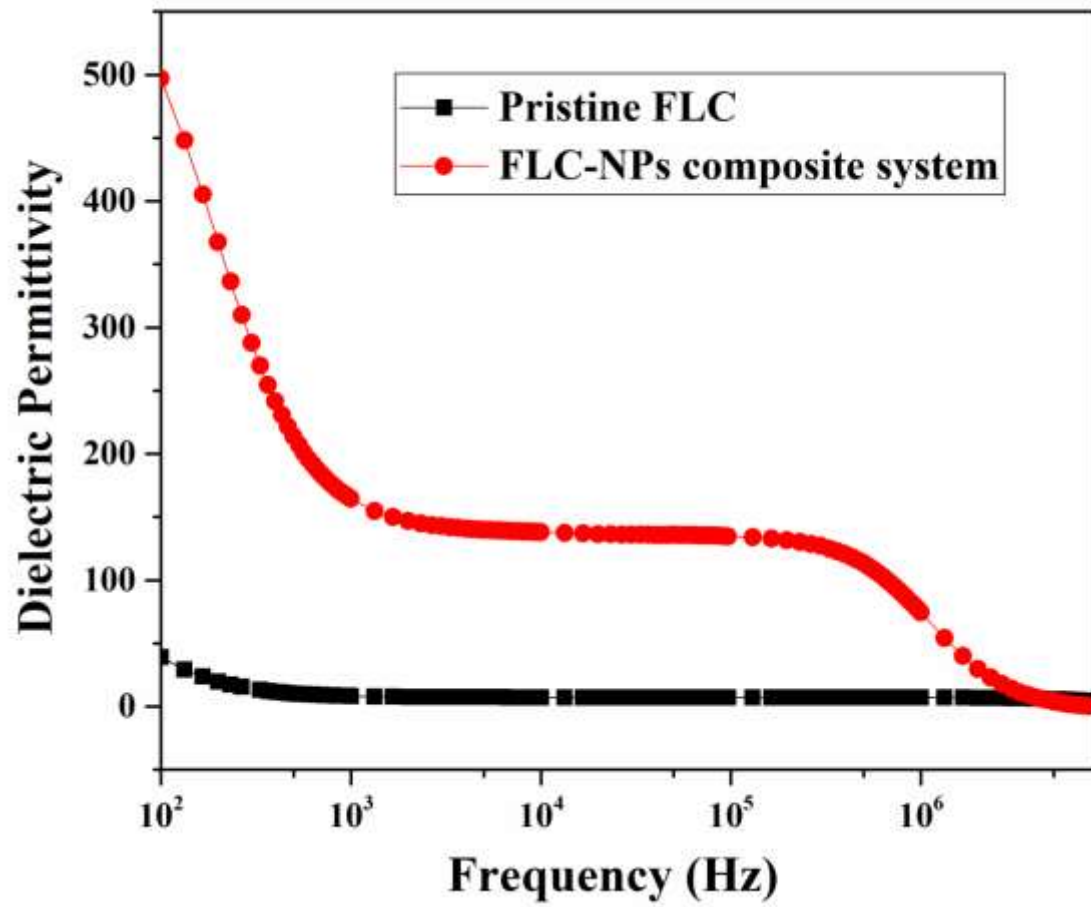
Fig. 1 Variation of dielectric permittivity with frequency for pristine FLC and FLC-NPs composite system.
