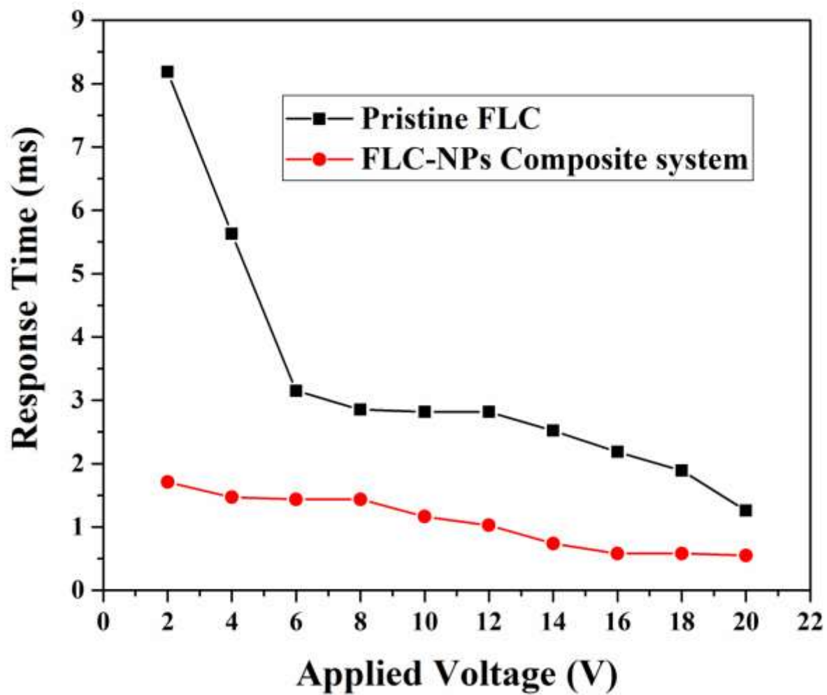
Fig. 2 Variation of response time with applied voltage for pristine FLC and FLC-NPs composite system.
