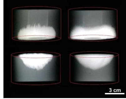
Figure 6: X-ray image of infiltrated samples (side view)
