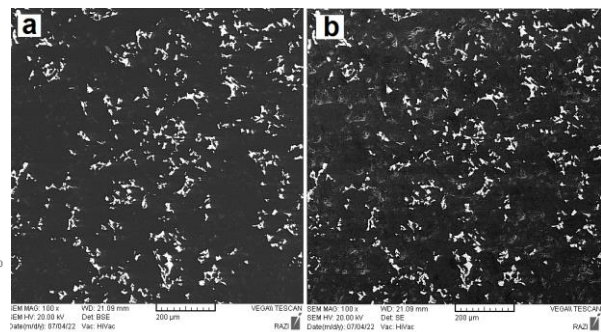
Figure 9: SEM micrographs of graphite/antimony composite at 100× magnification: (a) backscattered electron mode (b) secondary electron mode
