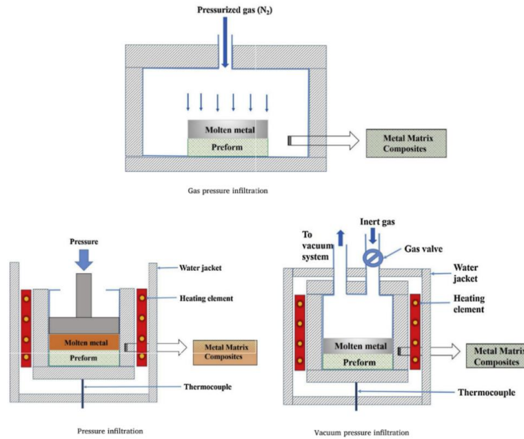
Figure 1: Some methods of melt penetration [2]
