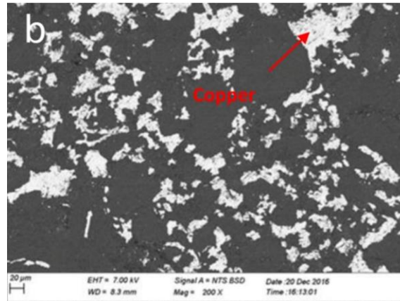
Figure 3: Microstructure of carbon/copper composite fabricated by melt penetration under mechanical stress [7]
