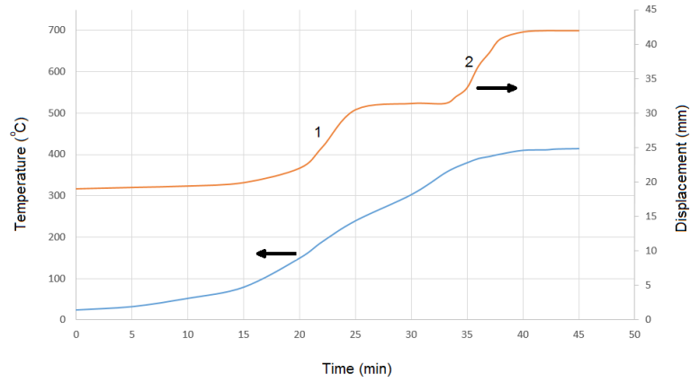
Figure 7: Temperature and displacement versus time graph for the SPS process for antimony infiltration
