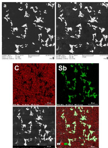
Figure 10: SEM micrographs of graphite/antimony composite at 400 \times magnification (a: backscattered electron mode, b: secondary electron mode) with elemental map of carbon and antimony
