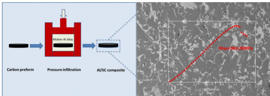
Figure 2: The process of infiltrating molten aluminum into a carbon body and the resulting microstructure [6]
