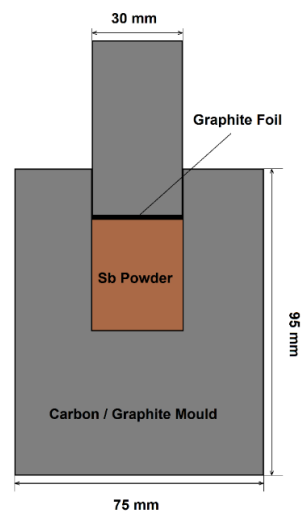
Figure 4: Components and dimensions of the mold used in antimony infiltration using the SPS method
