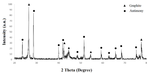
Figure 8: X-ray diffraction pattern of graphite/antimony composite
