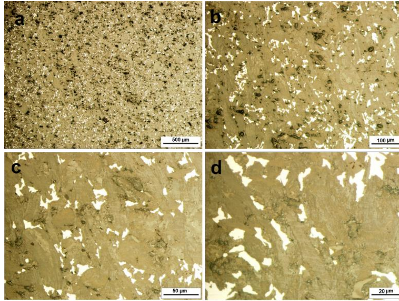
Figure 13: Optical micrographs of graphite/antimony composite at (a) 50×, (b) 200×, (c) 500× and (d) 1000× magnification
