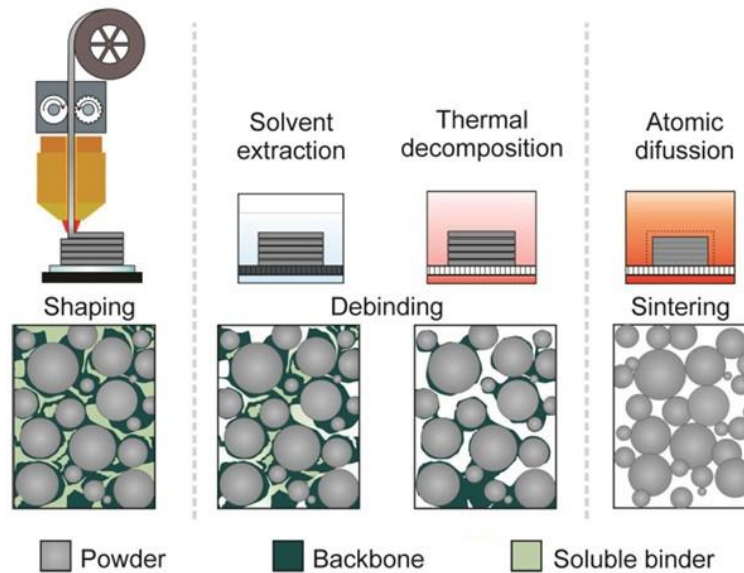
Figure 1. Schematic representation of the shaping, debinding, and sintering
