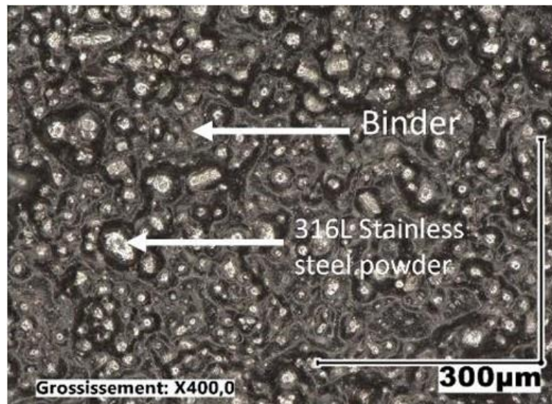
Figure 4. Optical microscope observation of part mixed with binder
