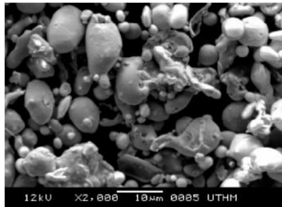
Figure 3. SEM image of SS 316L
