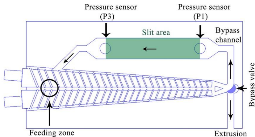
Figure 5. Schematic illustration of the Minilab for rheological characterization of the zirconia feedstocks
