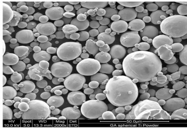
Figure 2. SEM image of titanium
