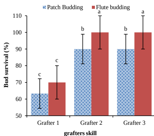
Fig. 8. Interactions between grafter's skill and budding methods on graft survival.
