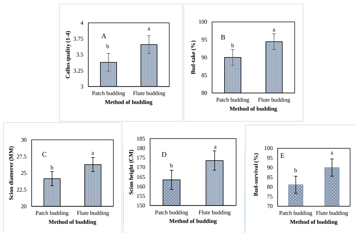
Fig. 2. The impact of flute and patch budding methods on callus quality (A), bud-take (B), scion diameter (C), scion growth (D), and bud survival (E). Bud survival calculated as (S/B) \times 100 , where S represents the number of surviving plants, and B denotes the number of bud-takes. Values with different letters denote statistical significance.
