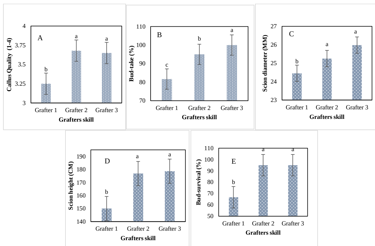
Fig. 3. The influence of grafter's skill on callus quality (A), bud-take (B), scion diameter (C), scion growth (D) and bud survival (E). Bud survival calculated as (S/B) \times 100 , where S represents the number of surviving plants, and B denotes the number of bud-takes. Values with different letters denote statistical significance.
