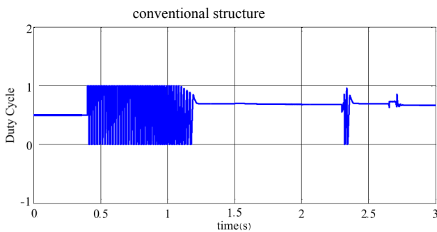
Fig. 14. The duty cycle variations of the suggested boost structure
