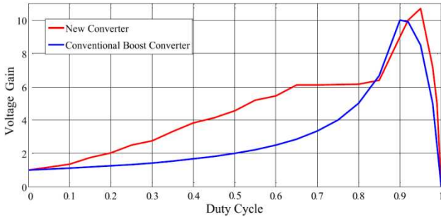
Fig. 8. The voltage gain of the conventional and suggested converter
