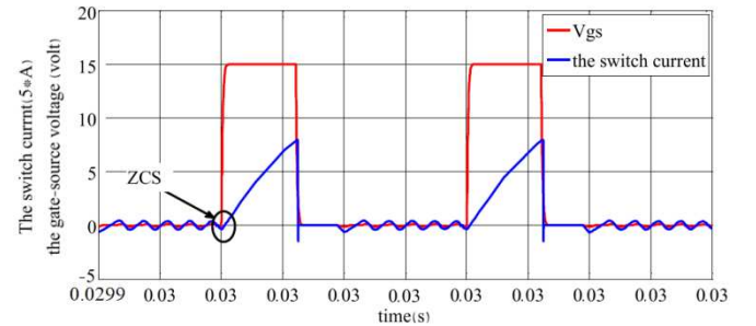
Fig. 5. The current of the power switch and gate driving signal
