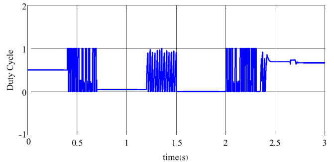
Fig. 12. The duty cycle variations of the conventional boost structure
