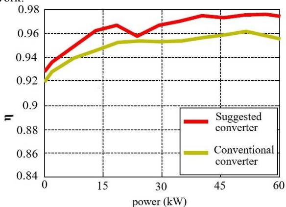
Fig. 16. Efficiency vs power
