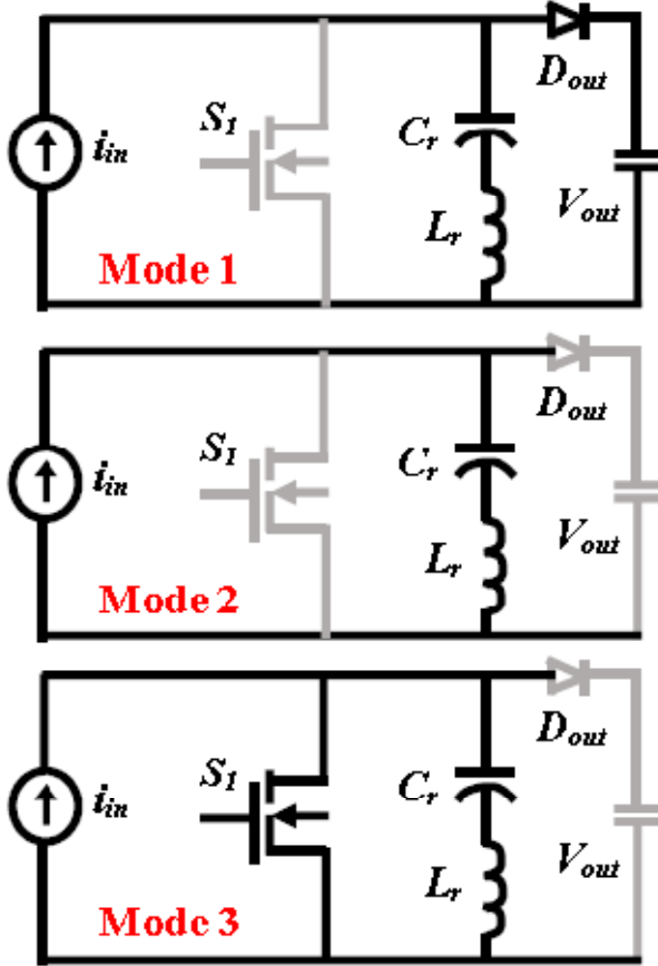
Fig. 2. The operating states and current paths in the converter
