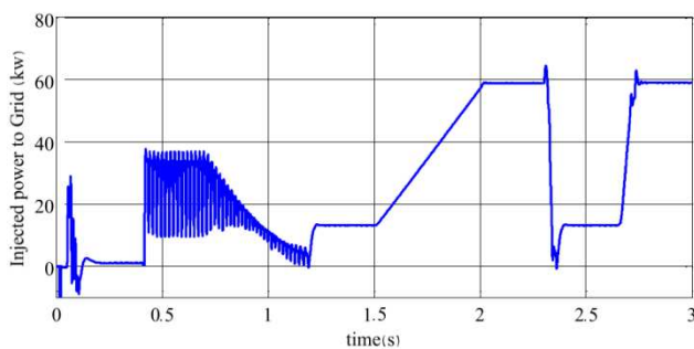
Fig. 15. The injected power from photovoltaic to the network under the suggested structure
