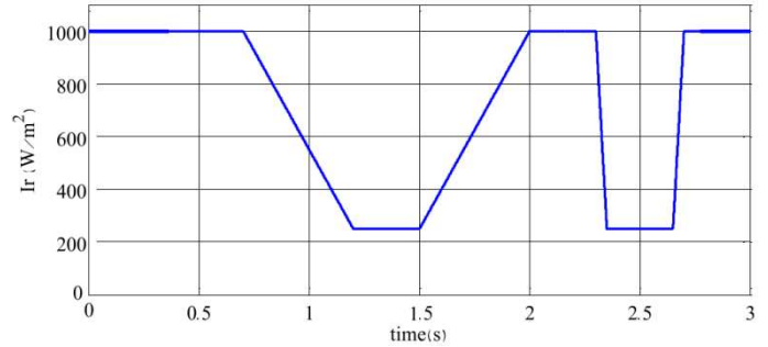
Fig. 10. The irradiance profile at the selected site
