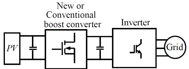
Fig. 11. The overall topology of the network-connected photovoltaic system
