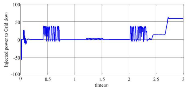
Fig. 13. The injected power from photovoltaic to the network under the suggested converter
