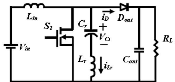
Fig. 1. The suggested high-gain DC-DC converter
