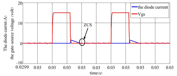
Fig. 4. The current of the diode and gate driving signal
