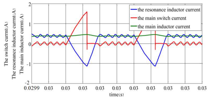
Fig. 6. The current of the power switch, resonance inductance, and input inductance
