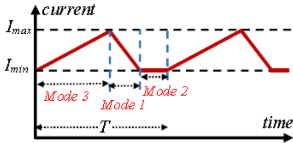
Fig. 3. Current changes in various operating modes
