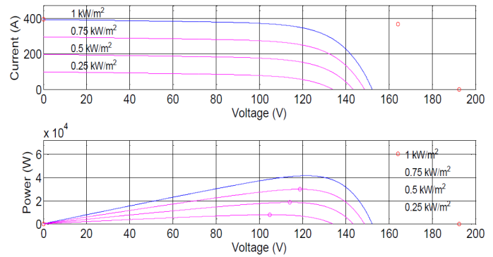
Fig. 9. The simulated characteristics of the PV module
