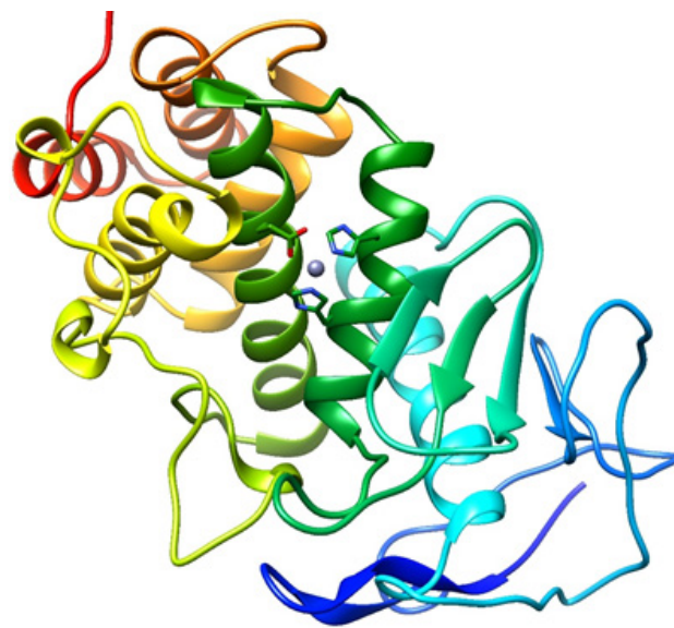
Fig. 1: 3-D structure of elastase (PDB ID: 3dbk)
