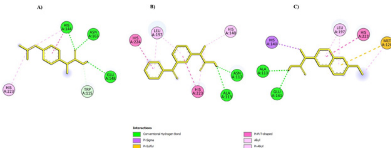
Fig. 2: Two dimensional views of NSAID/bacterial elastase complexes. A), B) and C) are, respectively, Ibuprofen, Ketoprofen and Naproxen
