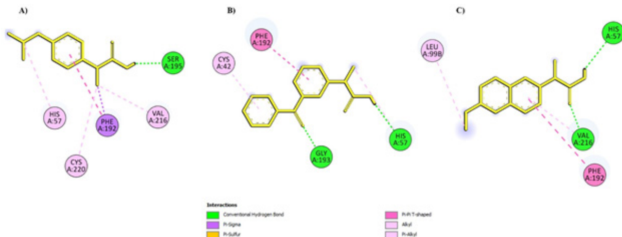
Fig. 3: Two dimensional views of NSAID/human elastase complexes. A), B) and C) are, respectively, Ibuprofen, Ketoprofen and Naproxen
