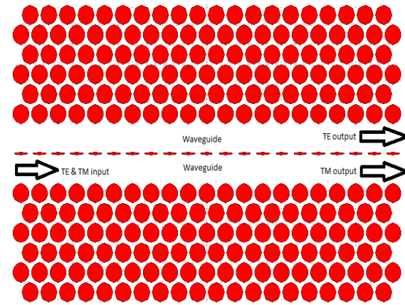
Fig. 4. 2D-geometry of the polarization splitter.
