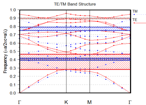
Fig. 3. Band diagram of both TE and TM modes.
