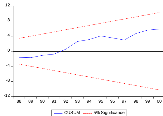
Fig 1. CUSUM Test
