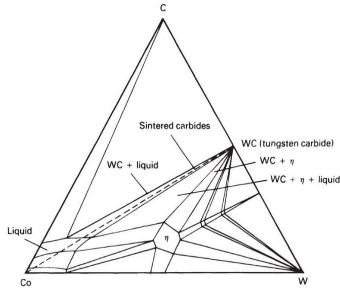
Fig. 5. Cobalt-tungsten-carbon ternary phase diagram [25].
