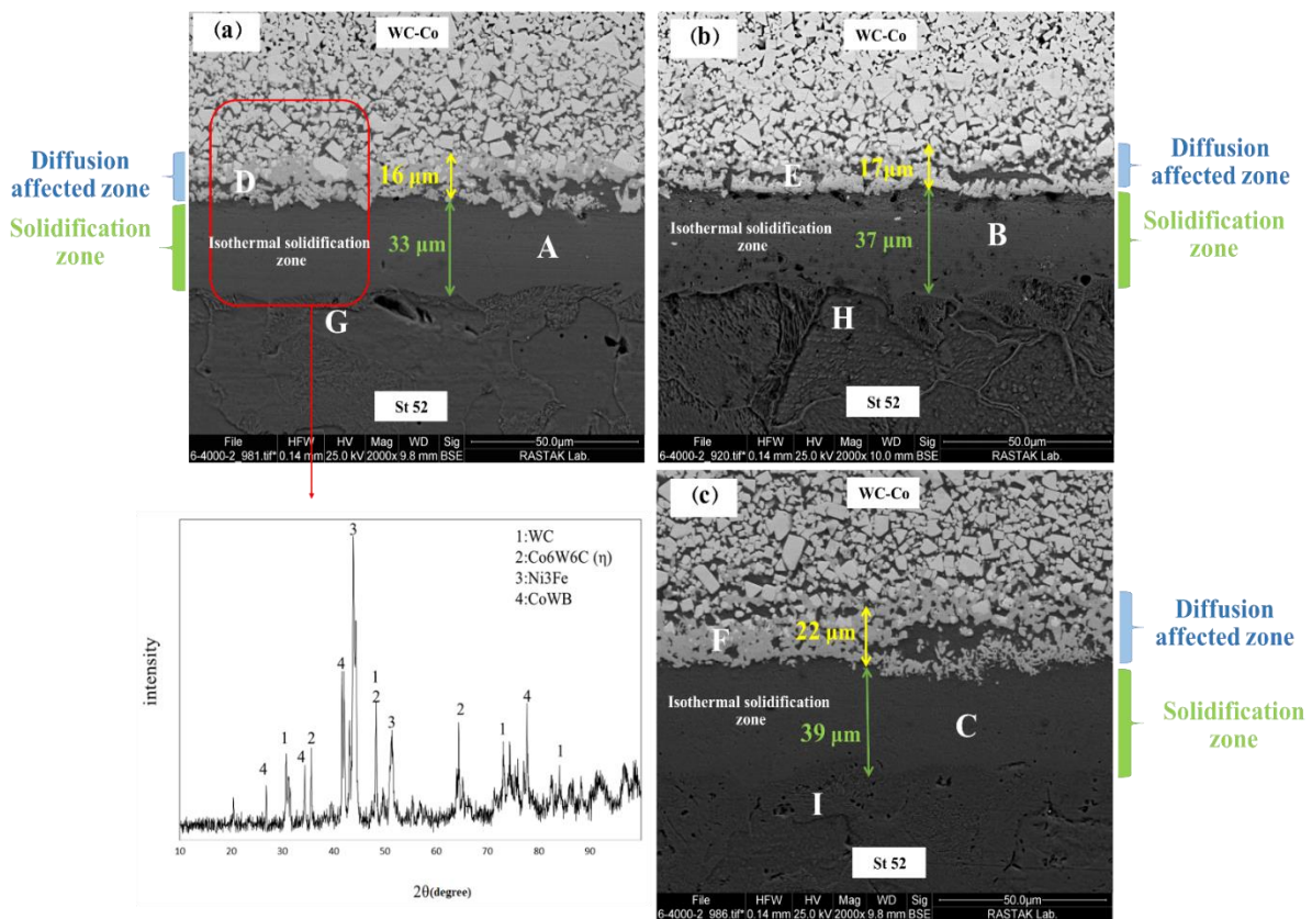
Fig. 6. SEM images of the bonded samples using BNi-2 interlayer at 1050 °C and holding times of a: 15, B: 30, and C: 45 min.
