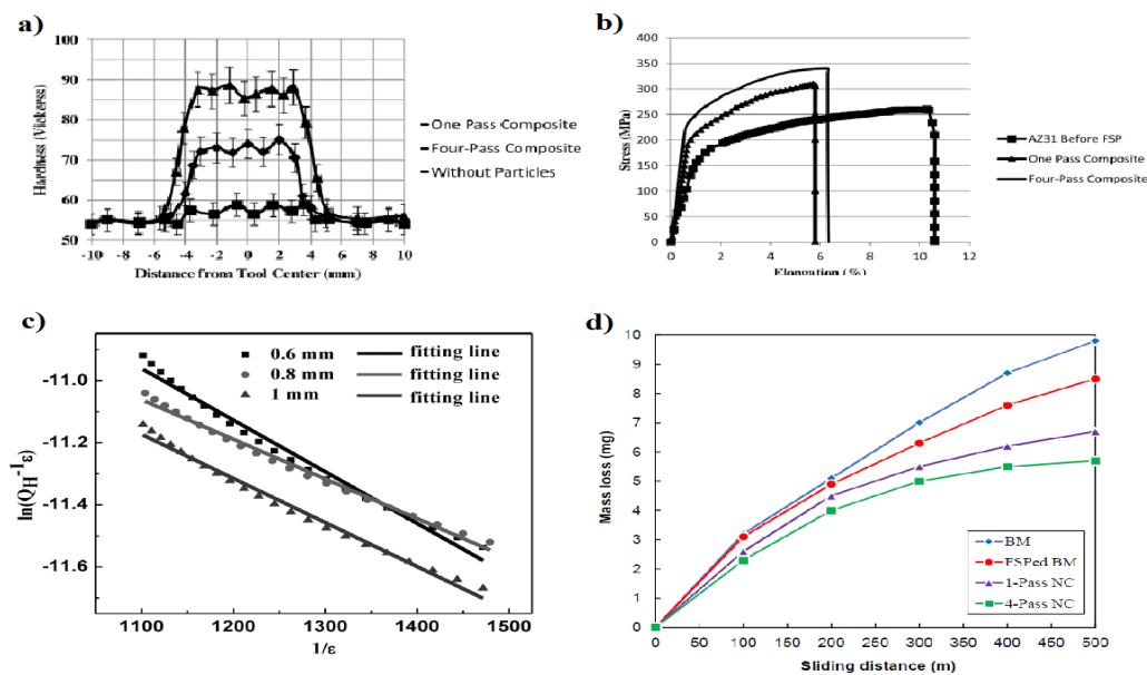
Fig. 7 (a) Hardness variations in the stir zone, (b) Stress variations before and after producing composite [23], (c) Damping-capacity dependence on the strain amplitude of ZrO 2 /Mg composites with different ZrO 2 amounts [35] and (d) Mass loss of the samples against sliding distance [36].
