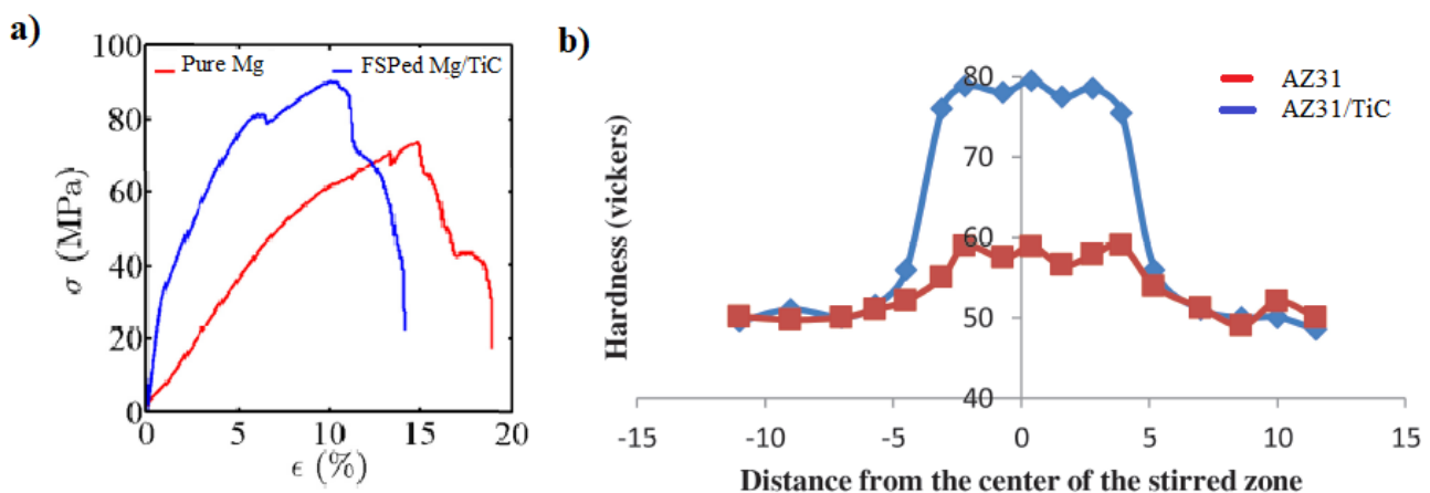
Fig. 10 a) Stress ( \sigma ) versus strain ( \epsilon ) plot obtained from the tensile testing of pure Mg and Mg+TiC composite fabricated by FSP [61], and b) Hardness Variation of AZ31 alloy and AZ31/TiC composite [62].
