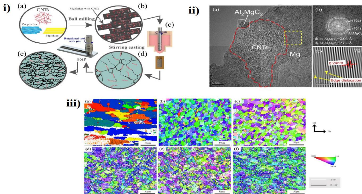
Fig. 11 i) Schematics for the fabrication procedures of the CNTs/Mg-6Zn composites: (a) the as-received materials, (b) the deposited CNTs with Mg chips by pre-treatments, (c) stirring casting, (d) microstructure morphology and CNTs distribution for the as-cast [70], and (e) the FSPed composites, ii) (a) High resolution TEM micrograph of Mg NC, (b) A digital SAEDP using a fast Fourier transform (FFT) of the area inside the white box in (a). (c) Inverse FFT image of the area inside the yellow box in (a) [71], The yellow T indicates the position and orientation of dislocation and iii) e EBSD IPF maps of different samples: (a) BM; (b) FSP sample; (c) AZ31/GNP composites; (d) FSP +50% rolling; (e) FSP +40% rolling + GNP; (f) FSP +50% rolling + GNP [75].
