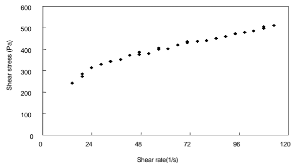
Fig. 2: A typical rheogram of low- calorie pistachio butter containing 0.01% RSG, no isomalt and the sucrose: pistachio paste ratio equal to 0.25
