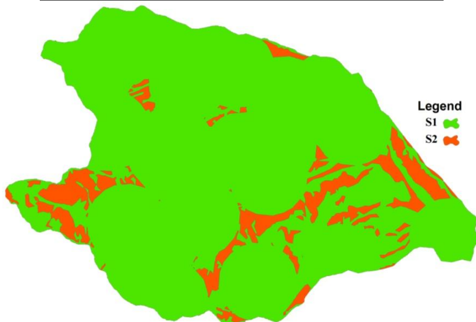
Fig. 17. The final model of water resource suitability
