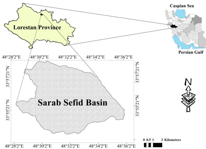
Fig. 1. Map of location of the study area, Sarab Sefid basin, Borujerd, Iran
