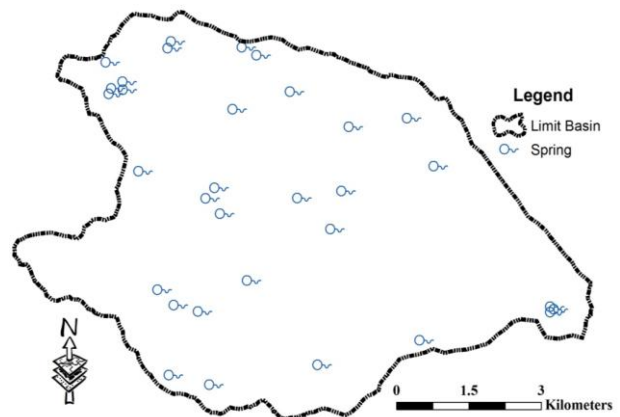
Fig. 8. The map of basin springs
