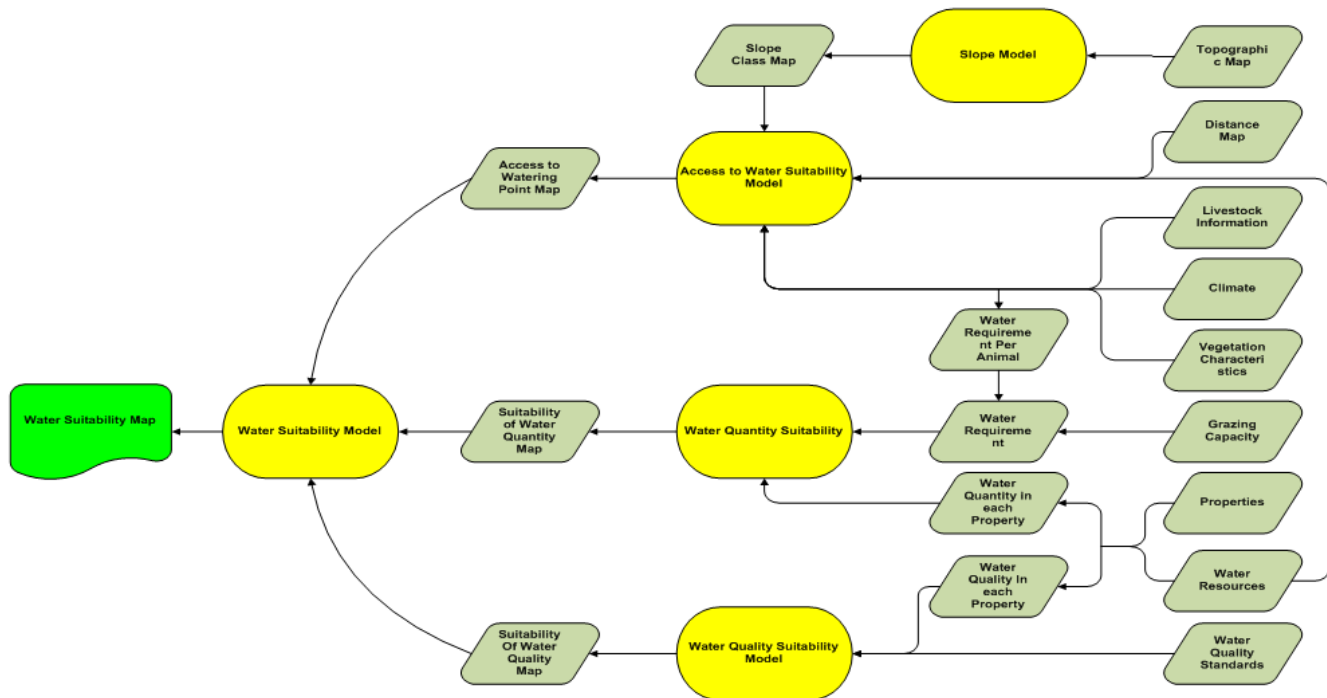
Fig. 10. Model for classification of water resources suitability
