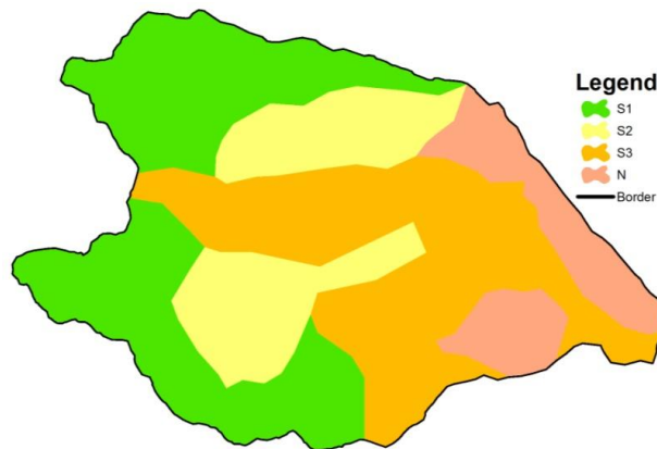
Fig. 11. Soil suitability categories map to erosion
