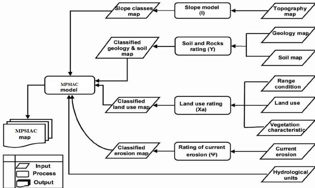
Fig. 5. Criteria in the MPSIAC erosion model (Amiri, 2009b)
