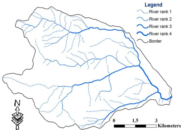
Fig. 7. The map of basin hydrological networks
