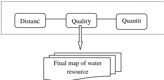
Fig. 9. The final model of water resource suitability for sheep grazing
