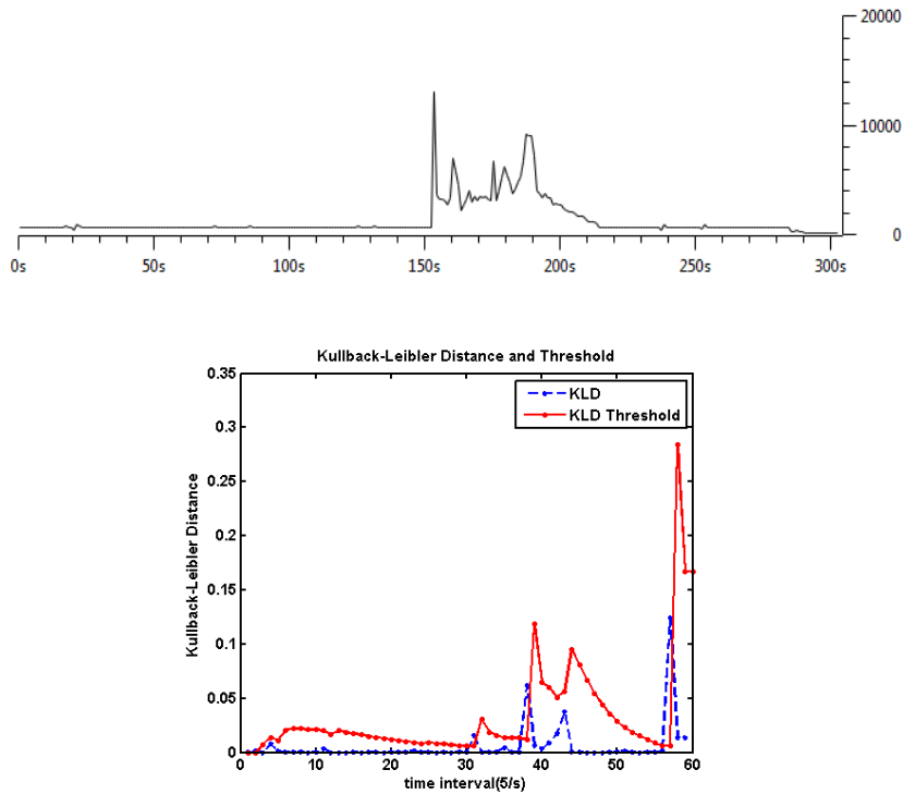
Fig. 12. Attack detection with traffic rate of 100 calls per second and attack mass of 100000 INVITE messages.
