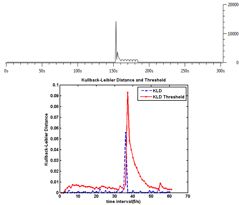
Fig. 10. Attack detection with traffic rate of 100 calls per second and attack mass of 10000 INVITE messages.
