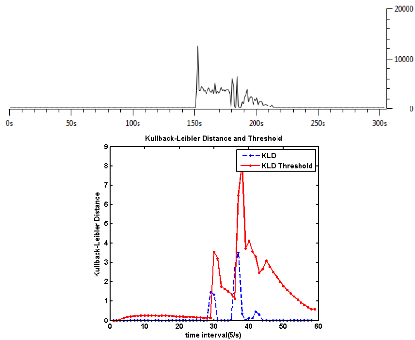
Fig. 6. Attack detection with traffic rate of 10 calls per second and attack mass of 1000000 INVITE messages.
