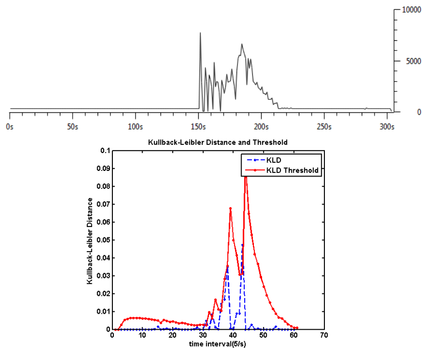
Fig. 9. Attack detection with traffic rate of 50 calls per second and attack mass of 1000000 INVITE messages.
