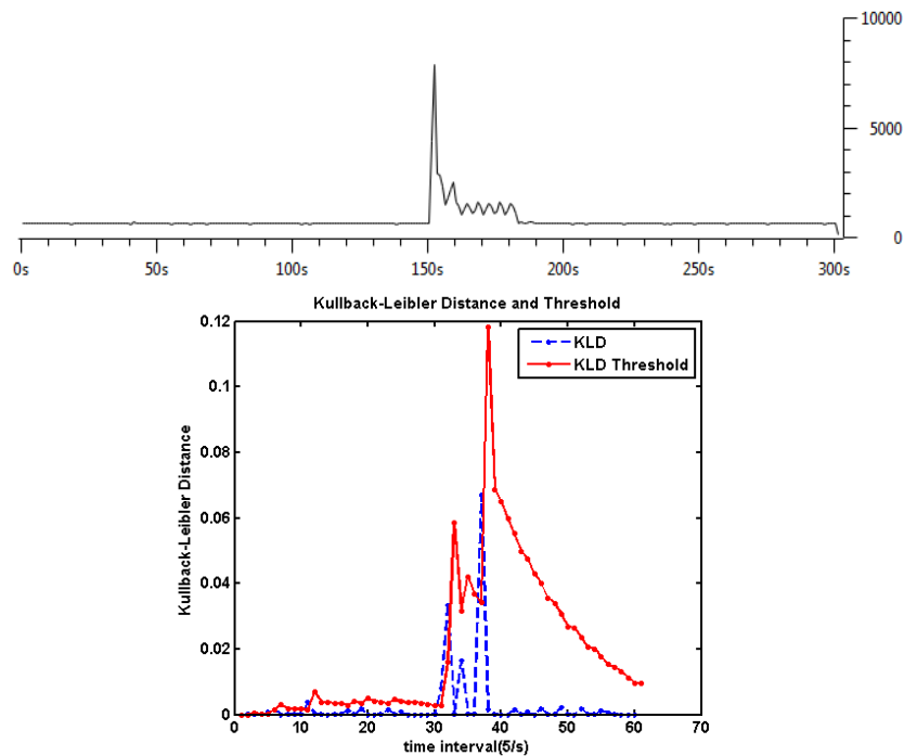
Fig. 11. Attack detection with traffic rate of 100 calls per second and attack mass of 100000 INVITE messages.
