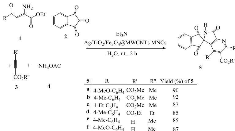
Scheme 1: Synthesis of functionalized spironinhydrines
