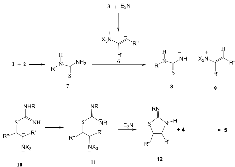
Scheme 2: Proposed mechanism for the formation of 5 .
