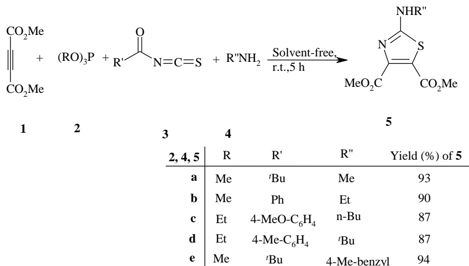
Scheme 1: Synthesis of imino thiazolane derivatives 5
