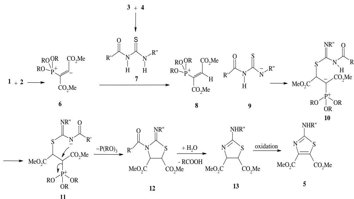
Scheme 2: proposed mechanism for the formation of 5
