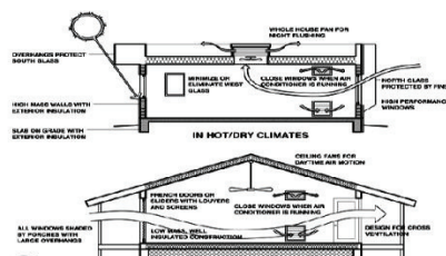
59 IN HOT/DRY CLIMATES In this climate air conditioning will always be required, but can be greatly reduced if building design minimize overheating.
