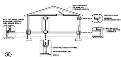
5 Carefully seal building to minimize infiltration and eliminate drafts, especially in windy sites (house wrap, weather stripping, tight windows).
