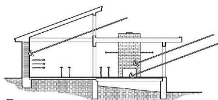
24 Use high mass interior materials like slab floors, high mass walls, and a stone fireplace to store winter passive heat and summer night 'coolth'.
