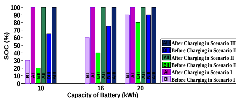
Figure (13): SOC changes of EVs battery before and after charging mode
