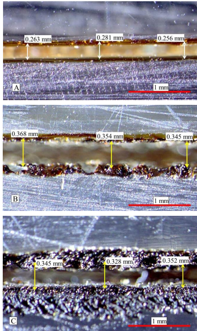
Figure1. Upper kerf width measurements at three points in the middle of the cut path where the cutting speed is steady. A) 2 mm thick, 45 W, 1200 mm/min. B) 6 mm thick, 45 W, 370 mm/min. C) 8 mm thick, 45 W, 300 mm/min. The dark zone surrounding the kerf is referring to HAZ and residual melt
