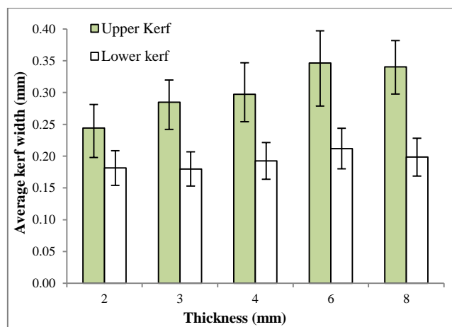
Figure9. The average upper and lower kerf width versus sheet thickness. The focused beam diameter was 0.1 mm
