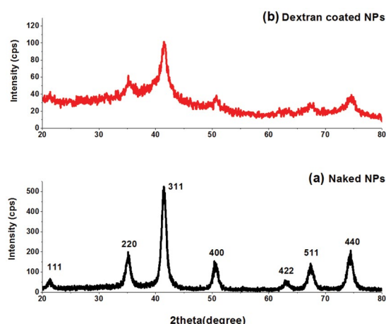
Fig. 1. XRD patterns of the electrodeposited samples.
