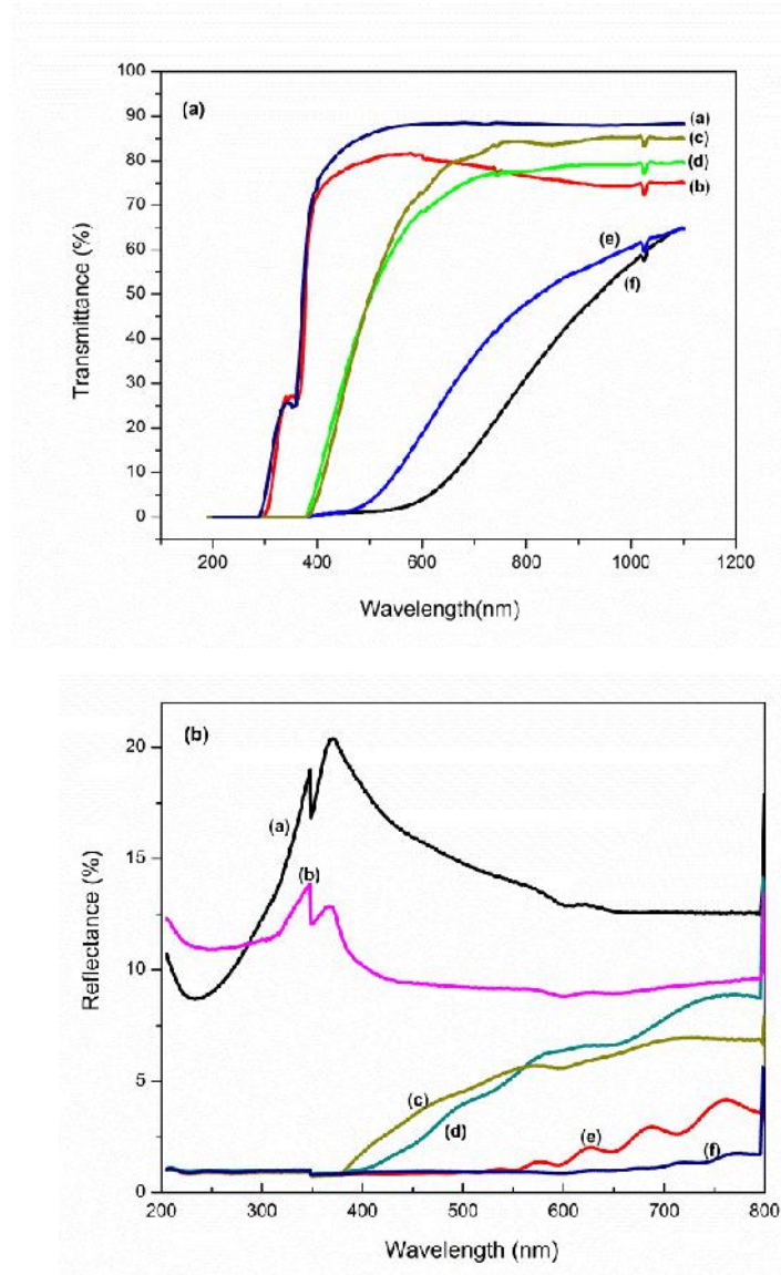
Fig. 6. Optical transmittance and reflectance spectra of ZnO a) seed layer, and hydrothermally synthesized NRs grown for b) 20, c) 40, d) 60, e) 120 and f) 240 min.
