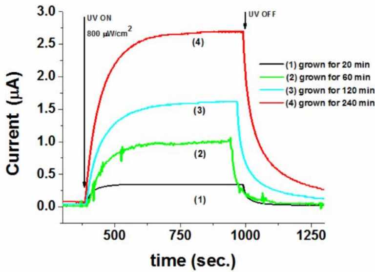
Fig.7. Ultra-violet detecting performance of ZnO nanorods grown at different times.
