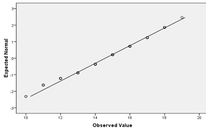
Figure 3: Q-Q plot of Scores
