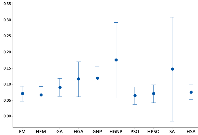
Fig. 18. Comparison of algorithms at VWS structure.
