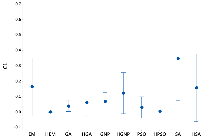
Fig. 11. Mean plot and LSD intervals at the 95 % confidence level for c_1 metric.
