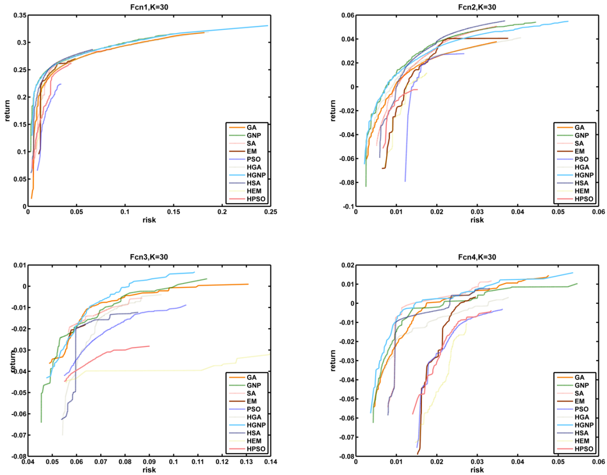
Fig. 10. Comparison of 10 algorithms on efficient frontiers, F_{cn} 1-4, K=30 .
