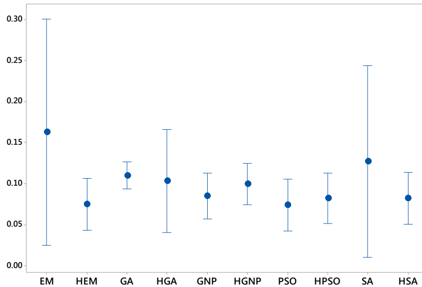
Fig. 17. Comparison of algorithms at MAD structure.
