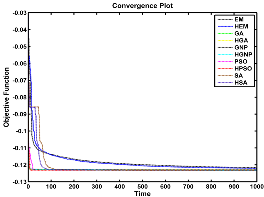
Fig. 7. Convergence plot for the proposed algorithms.
