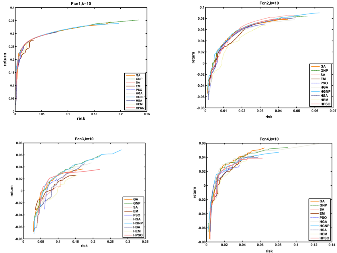
Fig. 8. Comparison of 10 algorithms on efficient frontiers, Fcn 1-4, K=10 .
