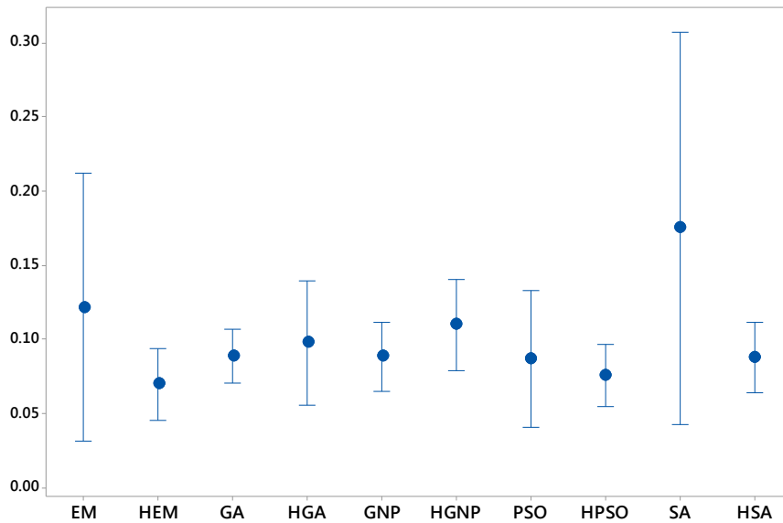
Fig. 19. Comparison of algorithms at K=10.
