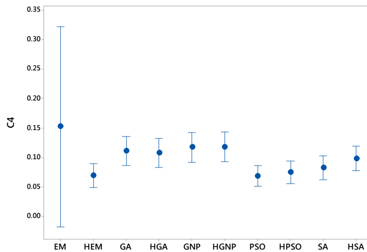
Fig. 14. Mean plot and LSD intervals at the 95 % confidence level for c_4 metric.
