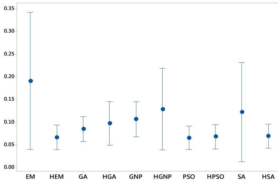
Fig. 20. Comparison of algorithms at K=20.
