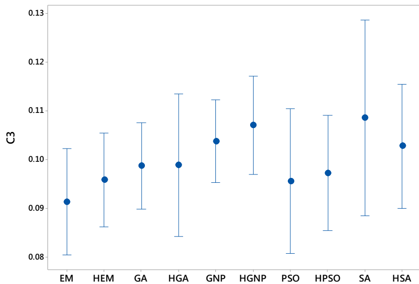
Fig. 13. Mean plot and LSD intervals at the 95 % confidence level for c_3 metric.
