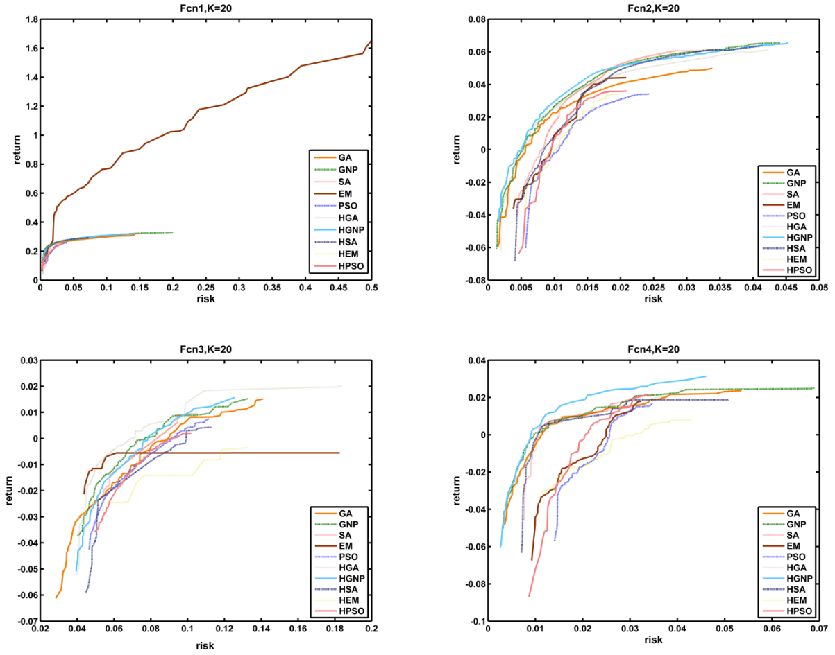
Fig. 9. Comparison of 10 algorithms on efficient frontiers, Fcn 1-4, K=20 .
