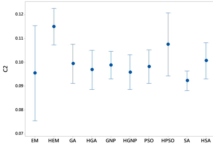
Fig. 12. Mean plot and LSD intervals at the 95 % confidence level for c_2 metric.
