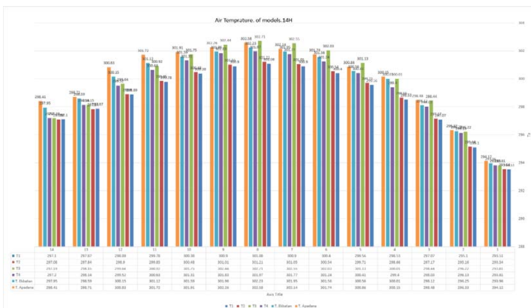
Fig. 4. Comparison of the Air temperatures of the models through 14 hours.
