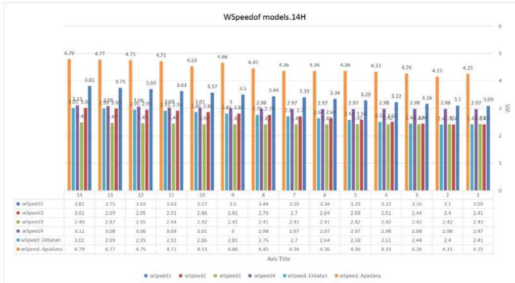
Fig.6. Comparison of the Wind Speed of the models through 14 hours
