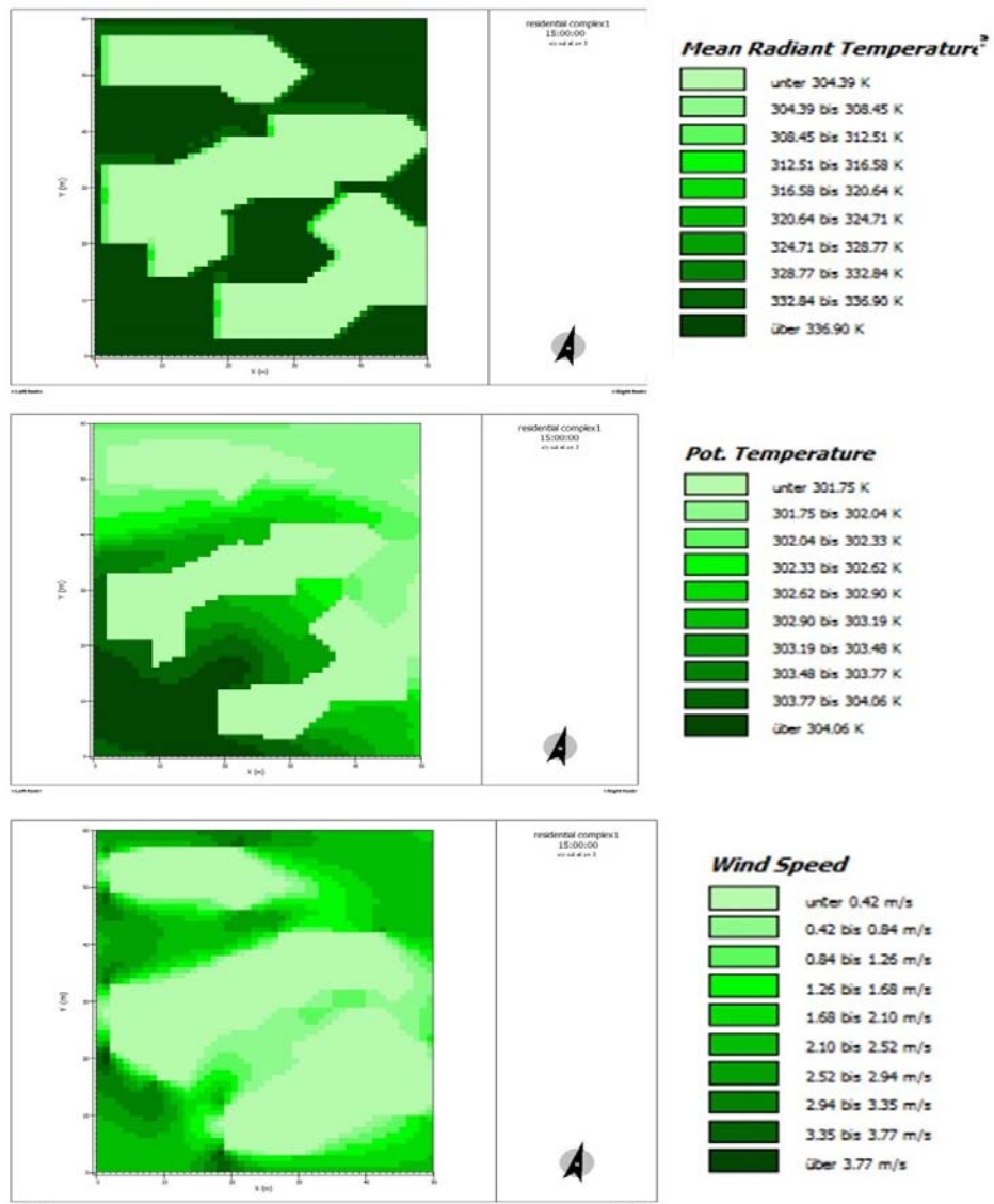
Fig. 7. visual situation of the simulated models at 15:00
