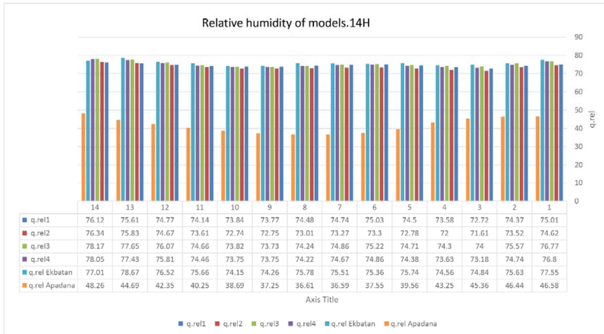
Fig. 5. Comparison of the Relative humidity of the models through 14 hours
