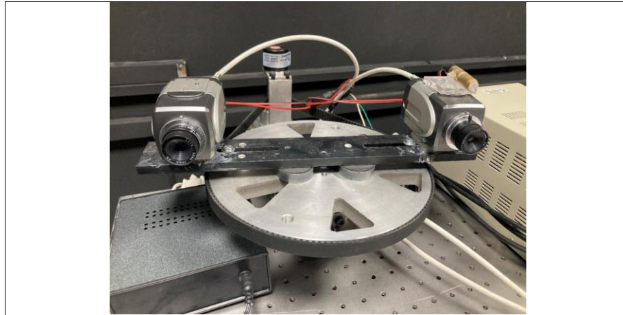
The laser scanner system built in this article
