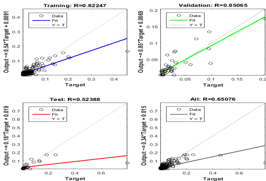
Fig. 5: Regression graph in the artificial neural network
