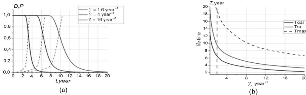
Fig.7 Reliabilities and life-time (a) of automotive hydraulic braking system depending on the rate of aging of the material and dependencies of change the characteristics of the life-time (b).
