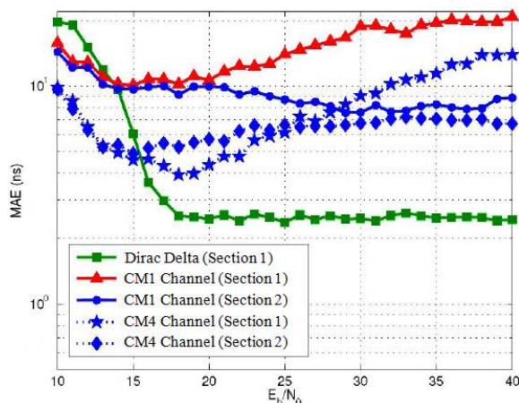
Fig.7. Performance of Synchronization Algorithm (Step: 6ns)
