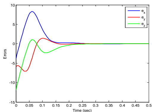
fig.6: Error trajectory between master and slave system
