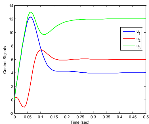
Fig.7. Control signals for synchronization of the master and slave systems.
