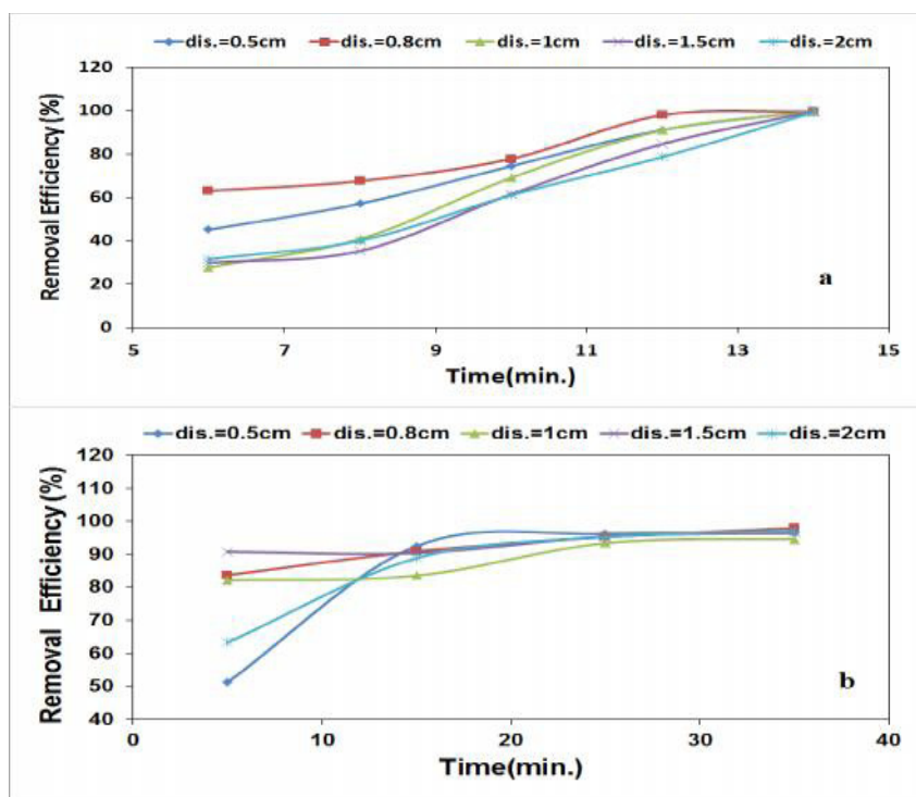
Figure 6. Effect of inter electrode distance on the efficiency of reactive red 24 dye removal using Fe (a) and Al (b) electrodes. Initial concentration of the dye = 100 \text{ mg L}^{-1} , current density = 10 \text{ mA cm}^{-2} , pH=7.2, [NaCl] concentration = 2.5 \text{ g L}^{-1} and temperature = 200\text{C} .
