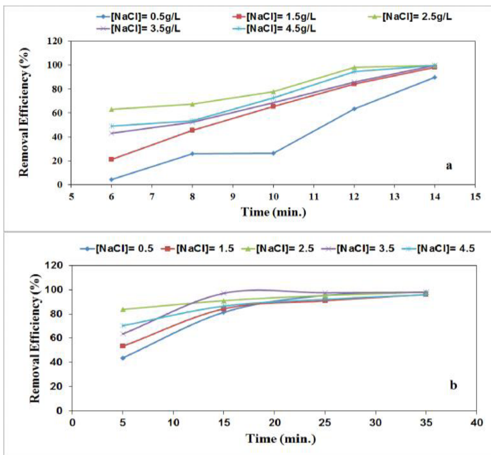
Figure 4. Effect of electrolyte concentration on the efficiency of reactive red 24 dye removal using Fe (a) and Al (b) electrodes. Initial concentration of the dye = 100 \text{ mg L}^{-1} , current density = 10 \text{ mA cm}^{-2} , pH=7.2, inter electrode distance = 0.8 cm and temperature = 200C.
