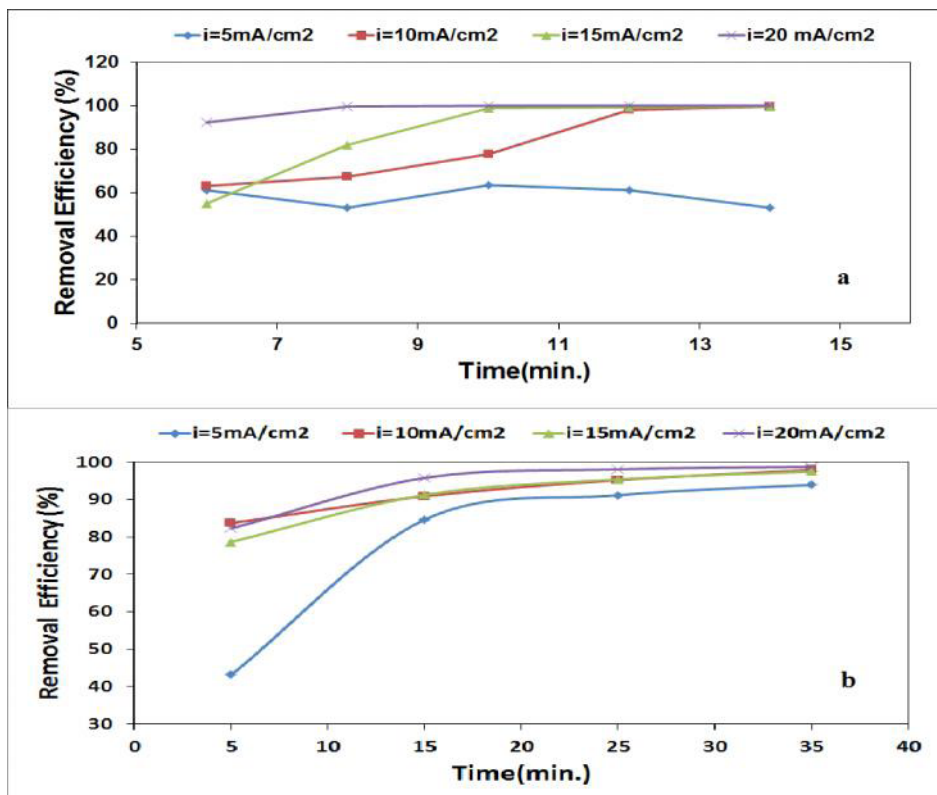
Figure 1. Effect of current density on the efficiency of reactive red 24 dye removal using Fe (a) and Al (b) electrodes. Initial concentration of the dye = 100 mg L -1 , [NaCl] concentration = 2.5 g L -1 , pH = 7.2, inter electrode distance = 0.8 cm and temperature = 200C
