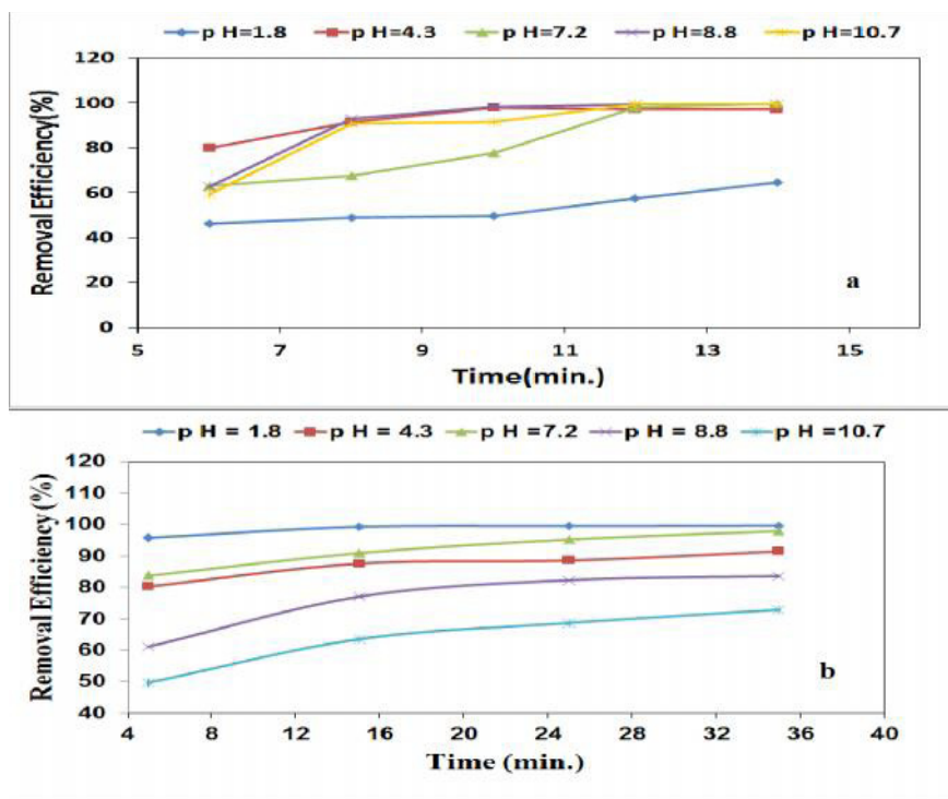
Figure 2. Effect of pH on the efficiency of reactive red 24 dye removal using Fe (a) and Al (b) electrodes. Initial concentration of the dye = 100 mg/L, [NaCl] concentration = 2.5 g L -1 , current density = 10 mA cm -2 , inter electrode distance = 0.8 cm and temperature = 200C
