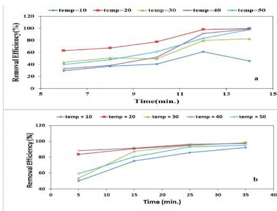
Figure 7. Effect of temperature on the efficiency of reactive red 24 dye removal using Fe (a) and Al (b) electrodes. Initial concentration of the dye = 100 mg/L, current density = 10 mA cm -2 , pH=7.2, [NaCl] concentration = 2.5 g L -1 and inter electrode distance = 0.8 cm.
