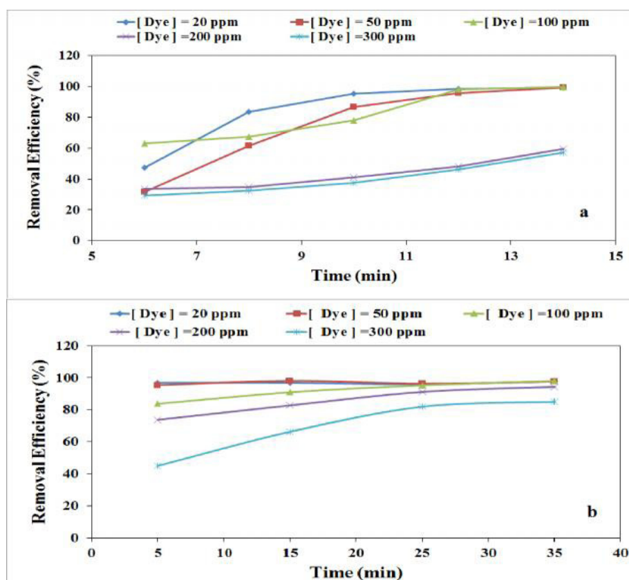
Figure 5. Effect of initial dye concentration on the efficiency of reactive red 24 dye removal using Fe (a) and Al (b) electrodes. [NaCl] concentration = 2.5 g L -1 , current density = 10 mA cm -2 , pH=7.2, inter electrode distance = 0.8 cm and temperature = 200C.
