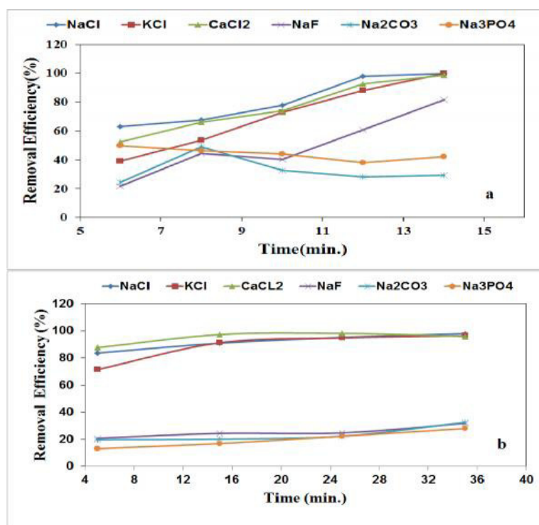
Figure 3. Effect of type of electrolyte on the efficiency of reactive red 24 dye removal using Fe (a) and Al (b) electrodes. Initial concentration of the dye = 100 mg L -1 , current density = 10 mA cm -2 , pH=7.2, inter electrode distance = 0.8 cm and temperature = 200C.
