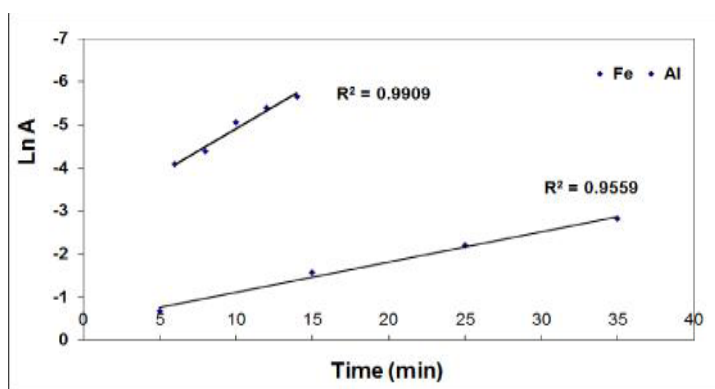
Figure 8. Relation between Ln A against the time for reactive red 24 dye removal using Fe (a) and Al (b) electrodes. Initial concentration of the dye = 100 \text{ mg L}^{-1} , current density = 10 \text{ mA cm}^{-2} , \text{pH}=7.2 , [\text{NaCl}] concentration = 2.5 \text{ g L}^{-1} , inter electrode distance = 0.8 \text{ cm} and temperature = 20^\circ\text{C} .
