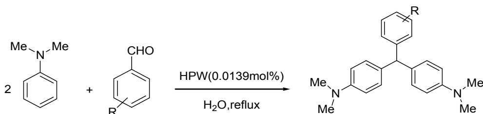
Scheme 1. HPW promoted synthesis of 4,4'-diaminotriarylmethanes in water.
