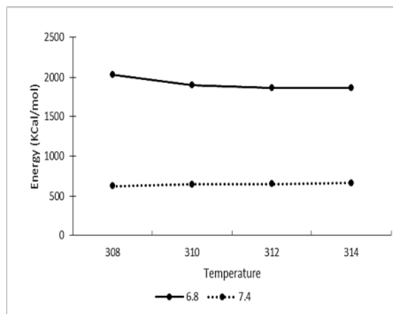
Fig. 2. Comparison of minimum energy level in different temperatures in BIO + force field.
