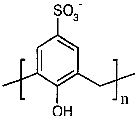
Fig. 1. Molecular structure of para-sulfonatocalix[n]arenes.
