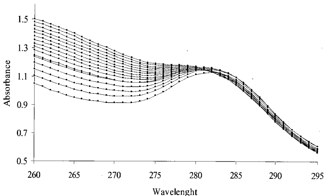
Fig. 2. Spectral changes of para-sulfonatocalix[n]arenes ( 9.90 \times 10^{-4} \text{ mol L}^{-1} ) in different metal ion concentration at 25 °C.
