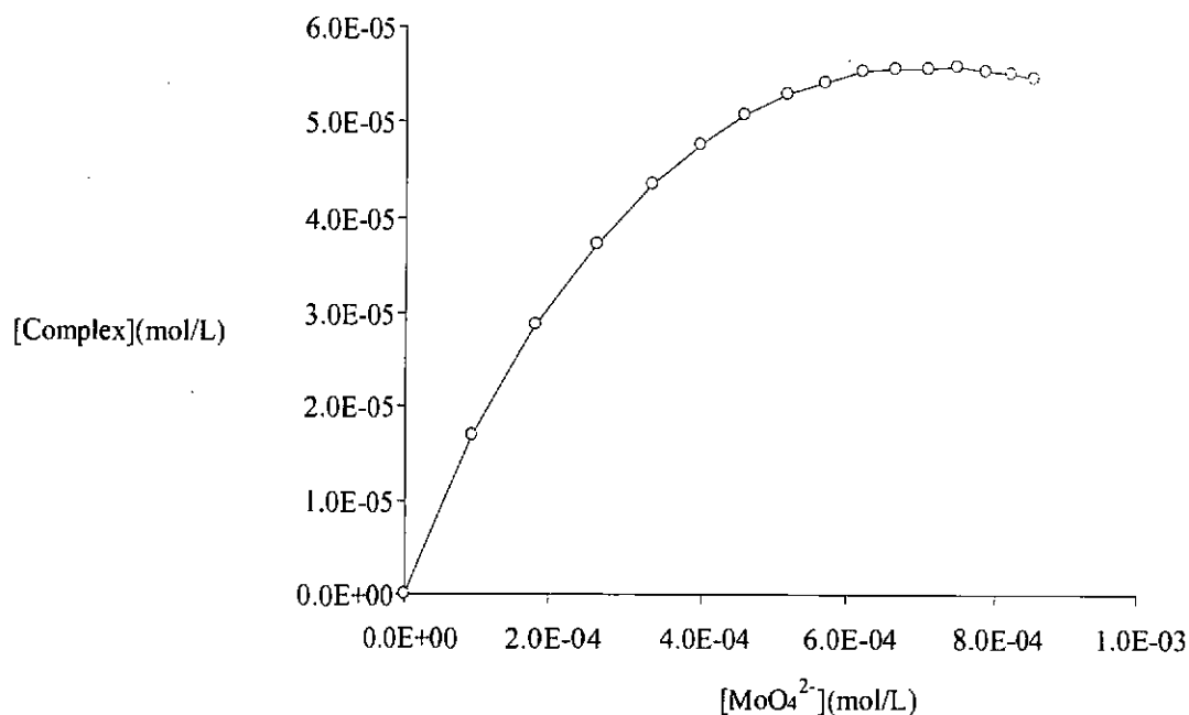
Fig. 4. Concentration profile of complex species at each titration point obtained by SQUAD program at 25 °C.
