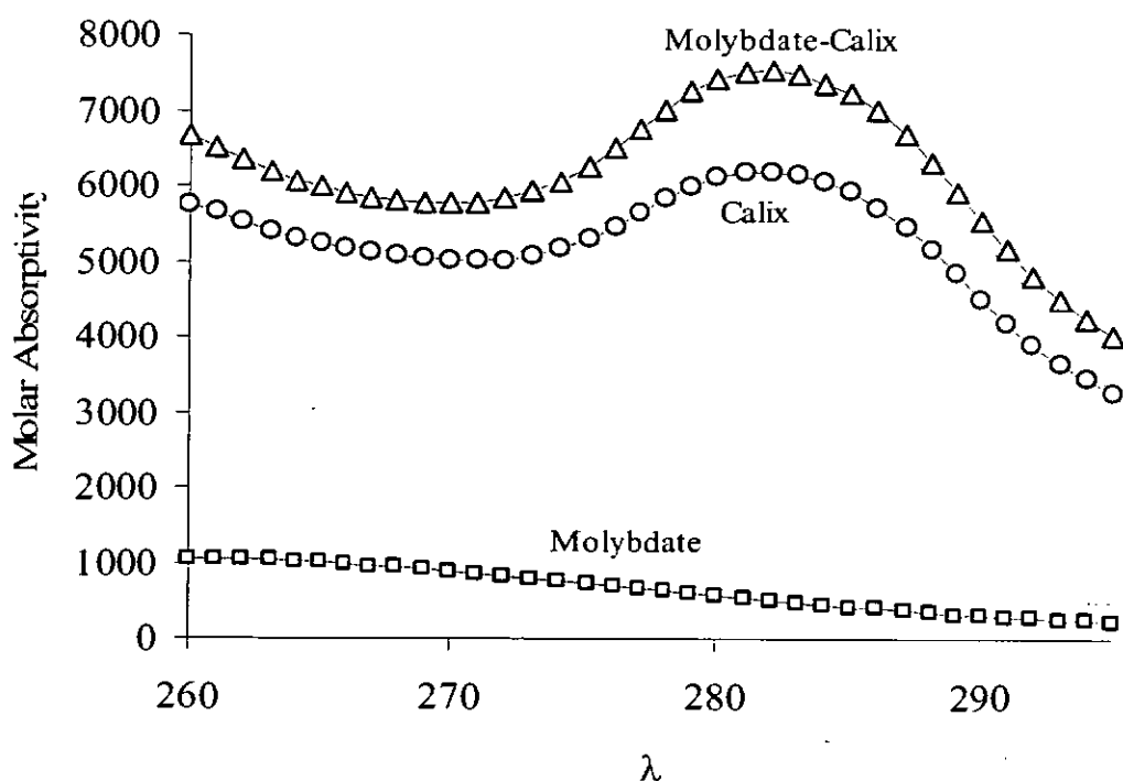
Fig. 3. Computed molar absorptivities of molybdenum ( \square ), para-sulfonatocalix [4] arene ( \circ ) and complex specie ( \Delta ) versus absorbance wavelength at 25 °C.
