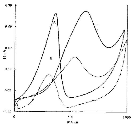
Fig. 3. Cyclic voltammograms of prepared Pt-Ru/PAN nanocomposite catalysts (insert A) and Pt-Ru/C catalysts (insert B) in 0.5 M \text{H}_2\text{SO}_4 and 0.5 M of methanol.
