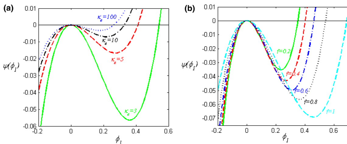
Fig. 4 The behavior of Sagdeev potential \psi(\phi) with respect to the electrostatic potential \phi , a for different values of electron suprathermality index \kappa_e with f = 0.8 , b for different values of ion
