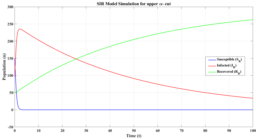
Figure 6: Evolution of populations at Upper \alpha -cut
