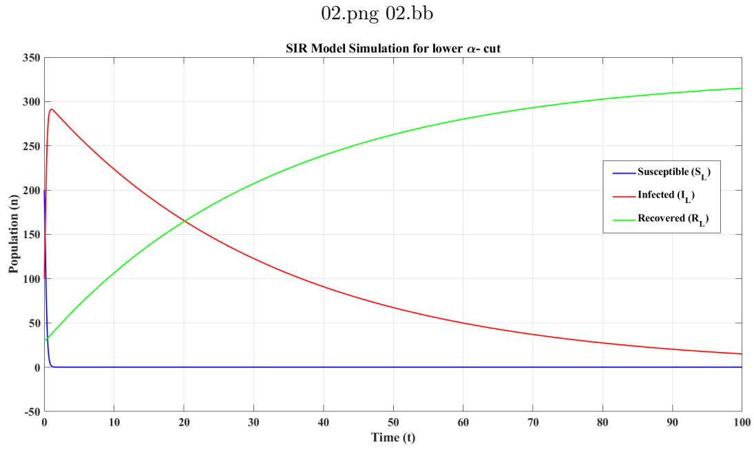
Figure 2: Dynamics of patients over time at support (lower alpha cut)
