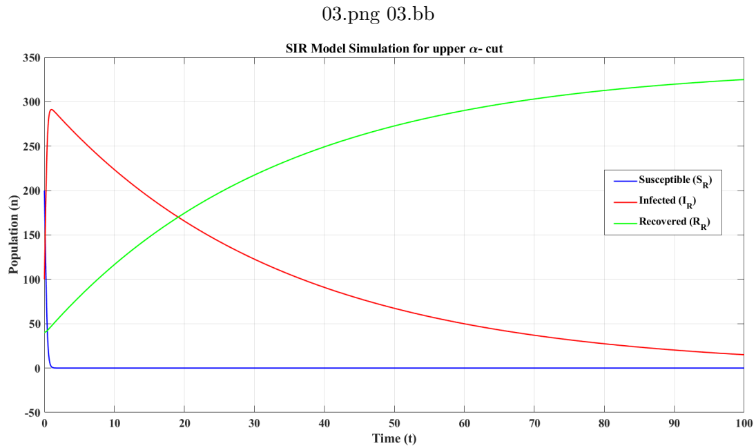
Figure 3: Dynamics of patients over time at support (Upper alpha cut)
