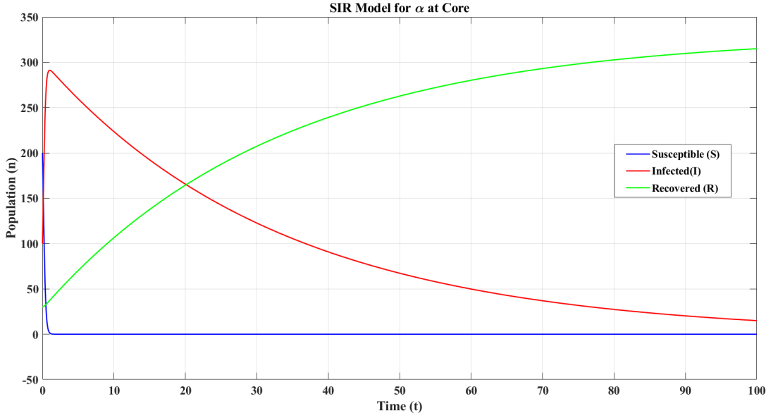
Figure 4: Dynamics of patients over time at the support at core
