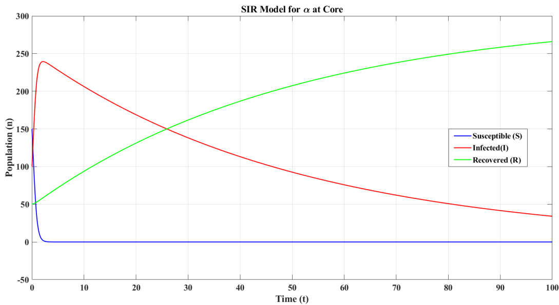
Figure 7: Dynamics of Fuzzy SIR model at core
