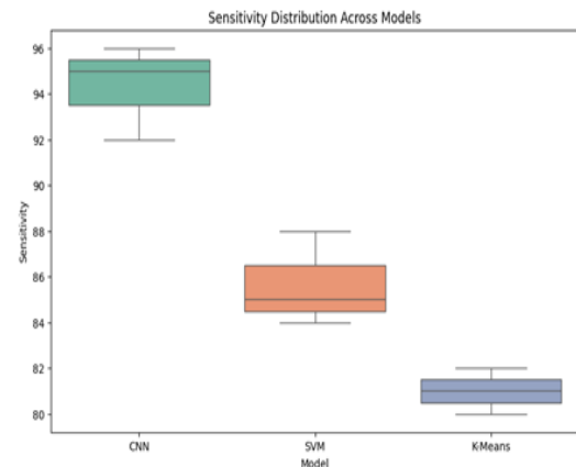
Figure 3. Box plot showing the Sensitivity Distribution Across Models (CNN, SVM, KMeans).
