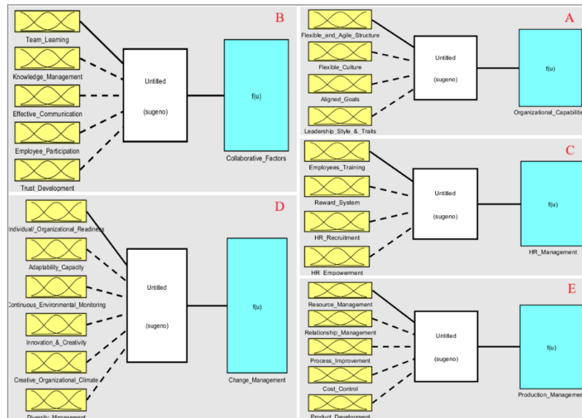
Fig. 5. Rule viewer
