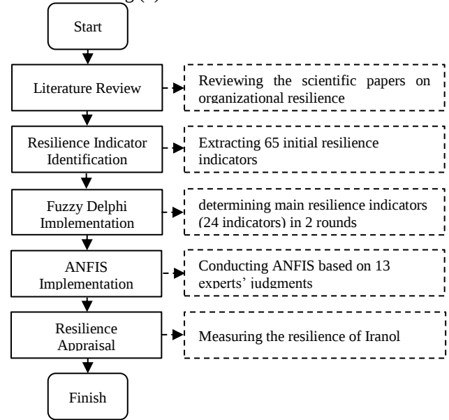
Fig. 1. Research framework
