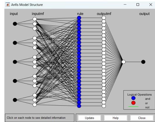
Fig. 8. ANFIS structure of the Main system
