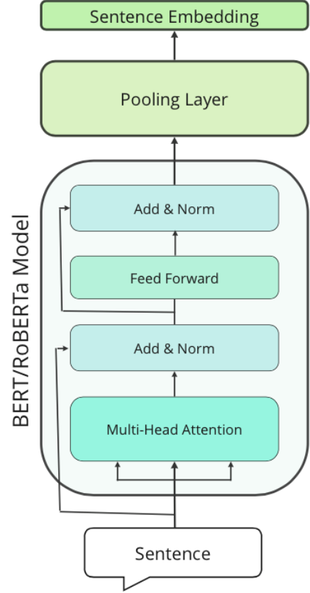
Figure 4 Sentence embedding
