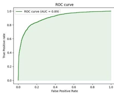
MVSA-Single-LDA
