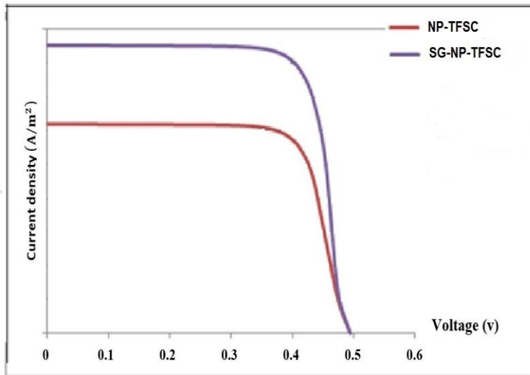
Fig. 4. Voltage-current diagram for NP-TFSC and SG-NP-TFSC
