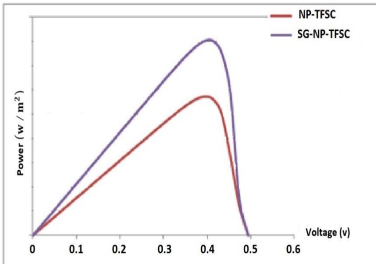
Fig. 5. Voltage-power diagram for NP-TFSC and SG-NP-TFSC
