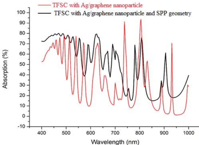
Fig. 3. The absorption profile of TFSC with Ag/graphene nanoparticle and TFSC with strips and grooves geometry
