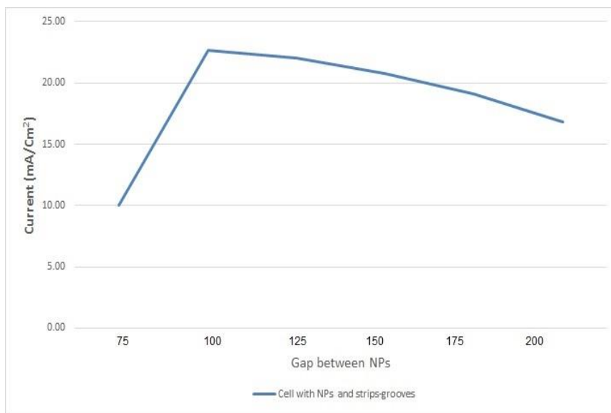
Fig. 2. Variation of J_{sc} versus the gap between nanoparticles
