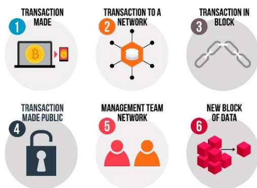
Fig. 1. Blockchain technology.
