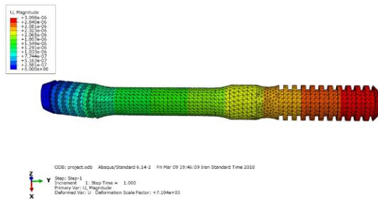
Fig. 10 Deformation of the bolt.
