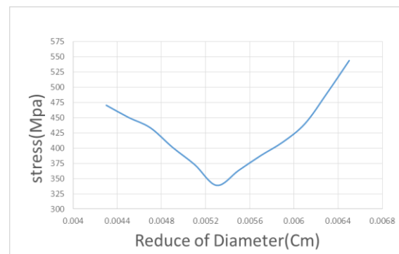
Fig. 12 Stress versus reduction of diameter.
