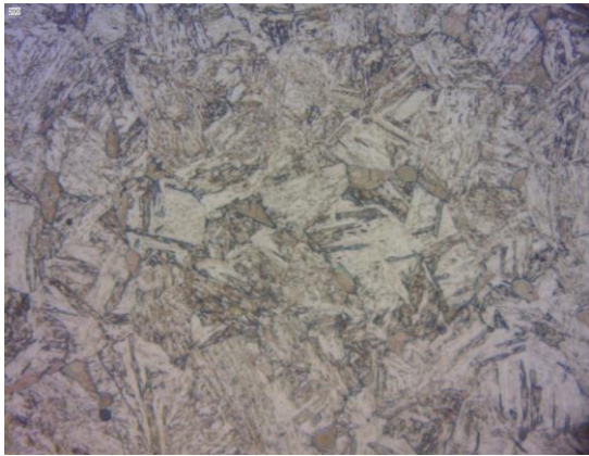
Fig. 7 Cross section fracture (200X).
