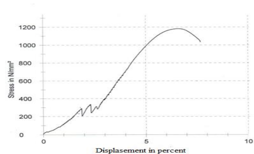
Fig. 3 Stress-strain diagram.
