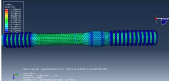
Fig. 9 Stress in the bolt caused by dynamic loading.
