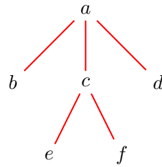
Figure 1. Multiple alleles
