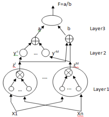
Fig.5. Neuro-Fuzzy network
