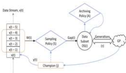
Fig. 7. Detection of botnets using genetic programming.
