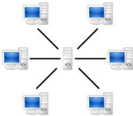
Fig. 1. Client-Server Architecture.
