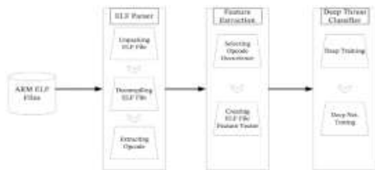
Fig. 9. Identification of botnets.
