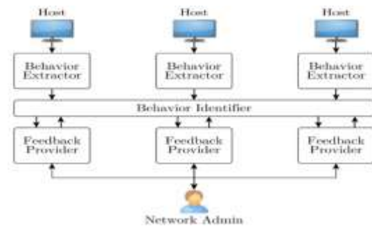
Fig. 8. The framework for identifying botnets.
