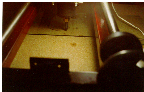
Fig. 2. Glazier on the instant of cutting a curve on a glass plate
