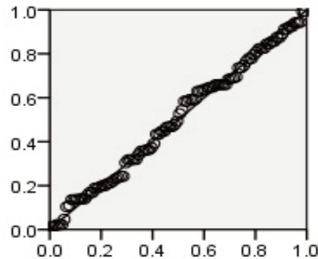
Figure 2. Standardized Residuals
